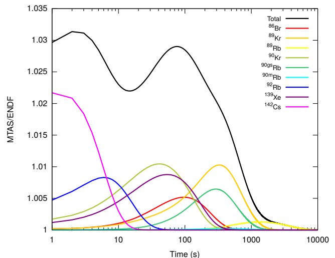
FIG. 3: color online The change of electromagnetic component of the decay heat calculated for ^{235}\text{U} + n_{\text{th}} fission. The different colors show the ratio of the decay heat calculated for MTAS and ENDF/B-VII.1 data (MTAS/ENDF) for individual nuclei. The black curve shows the total change.
