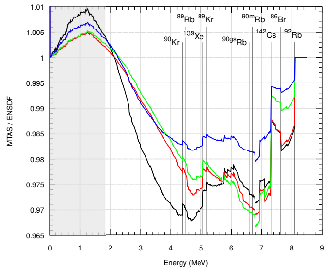
FIG. 5: color online Ratio of the calculated \overline{\nu}_e energy distribution from the MTAS measurement and data contained in the ENSDF database, designated for the most important nuclear fuel types, ^{235}\text{U} (black), ^{238}\text{U} (blue), ^{239}\text{Pu} (red), and ^{241}\text{Pu} (green). The shaded area denotes energies below the inverse \beta -decay threshold. Vertical lines indicate the Q_\beta values of the measured nuclei.
