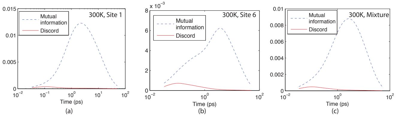
FIG. 2: (Color online) Mutual information I(A; B) and quantum discord D(A; B) with system A as site three and system B as sites one and six. The figure plots these quantities at physiological temperature ( 300^\circ\text{K} ) as a function of time when the initial state is (a) a pure state at the first site, (b) a pure state at the sixth state, (c) an equal mixture of the two previous states. In each of the above figures, the quantum discord is a non-negligible fraction of the total correlation during the first picosecond.
