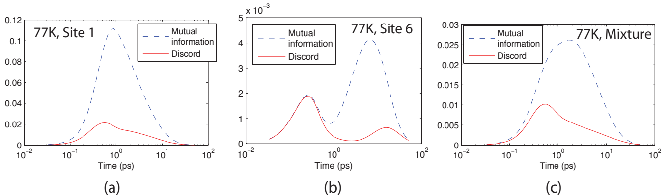
FIG. 3: (Color online) Mutual information I(A; B) and quantum discord D(A; B) with system A as site three and system B as sites one and two. The figure plots these quantities at cryogenic temperature ( 77^\circ\text{K} ) as a function of time when the initial state is (a) a pure state at the first site, (b) a pure state at the sixth state, (c) an equal mixture of the two previous states. In each of the above cases, the quantum discord is a significant fraction of the total correlation during the first picosecond. In fact, for the second case, the quantum discord contributes nearly all of the total correlation during the first picosecond.
