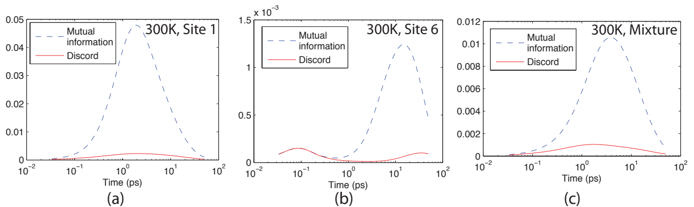
FIG. 4: (Color online) Mutual information I(A; B) and quantum discord D(A; B) with system A as site three and system B as sites one and two. The figure plots these quantities at physiological temperature (300°K) as a function of time when the initial state is (a) a pure state at the first site, (b) a pure state at the sixth state, (c) an equal mixture of the two previous states. In each of the above cases, the quantum discord contributes a fraction of the total correlation during the first picosecond. In the second case, it again contributes nearly all of the total correlation during the first picosecond.
