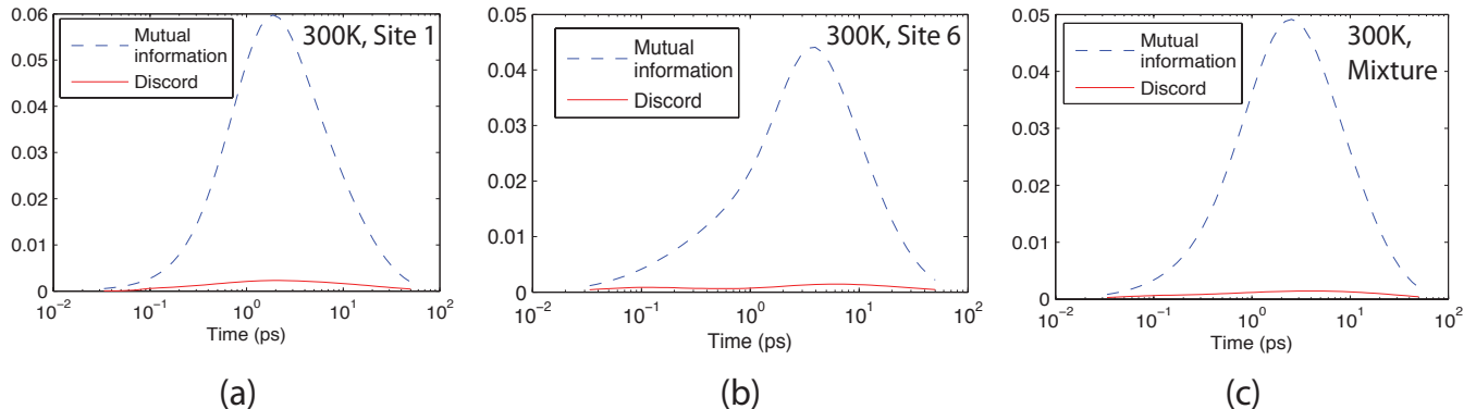
FIG. 6: (Color online) Mutual information I(A; B) and quantum discord D(A; B) with system A as site three and system B as all other sites (1-2, 4-7). The figure plots these quantities at physiological temperature ( 300^\circ\text{K} ) as a function of time when the initial state is (a) a pure state at the first site, (b) a pure state at the sixth state, (c) an equal mixture of the two previous states. The quantum discord does not contribute a large fraction of the total correlation here.
