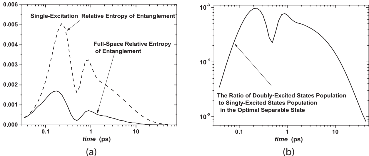
FIG. 7: (a) This figure simulates the dynamics of the FMO complex at 77^\circ\text{K} and calculates both the single-excitation relative entropy of entanglement and the full relative entropy of entanglement for A = 1, 6 and B = 3 . (b) The ratio of the number of doubly-excited states to the number of singly-excited states in the optimal separable state for the relative entropy of entanglement is rather small.
