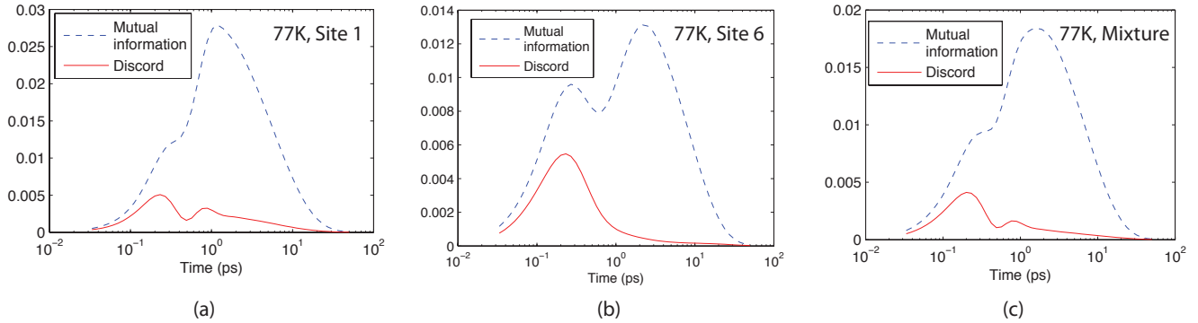
FIG. 1: (Color online) Mutual information I(A; B) and quantum discord D(A; B) with system A as site three and system B as sites one and six. The figure plots these quantities at cryogenic temperature ( 77^\circ\text{K} ) as a function of time when the initial state is (a) a pure state at the first site, (b) a pure state at the sixth state, (c) an equal mixture of the two previous states. In each of the above plots, the quantum discord is a significant fraction of the total correlations during the first picosecond.
