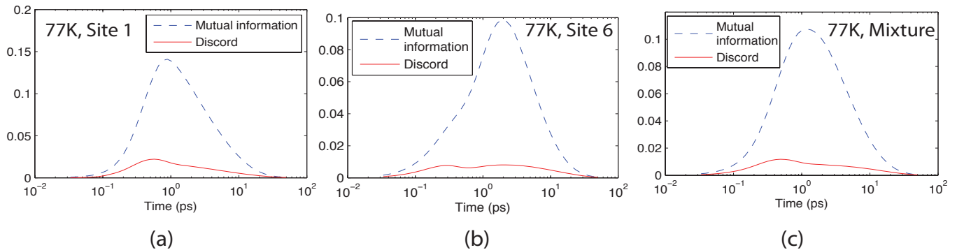
FIG. 5: (Color online) Mutual information I(A; B) and quantum discord D(A; B) with system A as site three and system B as all other sites (1-2, 4-7). The figure plots these quantities at cryogenic temperature ( 77^\circ\text{K} ) as a function of time when the initial state is (a) a pure state at the first site, (b) a pure state at the sixth state, (c) an equal mixture of the two previous states. The quantum discord contributes a significant fraction of the total correlation during the first picosecond.
