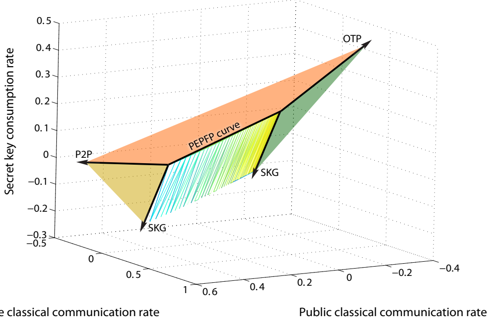
Fig. 4 (Color online) The private dynamic capacity region for a 1 \rightarrow 10 cloning channel. The region exhibits a non-trivial resource trade-off only on the surface below the PEPPF trade-off curve in the direction of secret key distribution.
