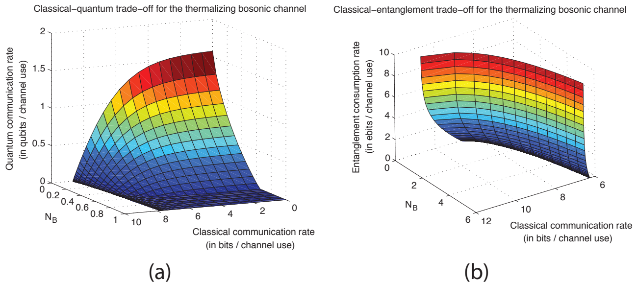
FIG. 5. (Color online) This figure displays the effect of increasing thermal noise (parametrized by N_B ) on the trade-off between (a) classical and quantum communication and (b) entanglement-assisted and unassisted classical communication. We cannot say whether any points in these regions are optimal because the capacity of the thermal channel is unknown (though, they are known if the minimum-output entropy conjecture is true [22, 23]).
