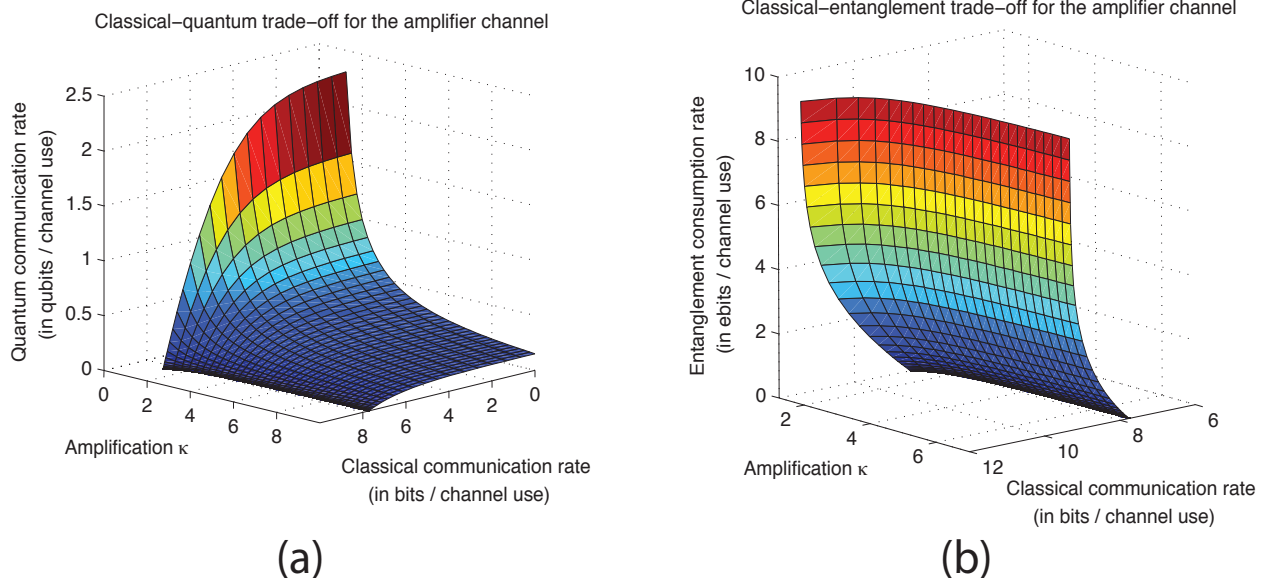
FIG. 6. (Color online) (a) Trade-off between classical and quantum communication for the bosonic amplifying channel with N_S = 200 and N_B = 0 for increasing values of the amplification parameter \kappa . (b) Trade-off between entanglement-assisted and unassisted classical communication for the same channel. For both trade-offs, more amplification degrades performance because it introduces too much noise.
