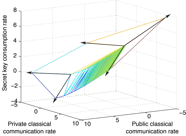
FIG. 4. (Color online) The private dynamic capacity region for a lossy bosonic channel with transmissivity \eta = 3/4 and mean input photon number N_S = 100 . The units for each kind of resource are bits per channel use.
