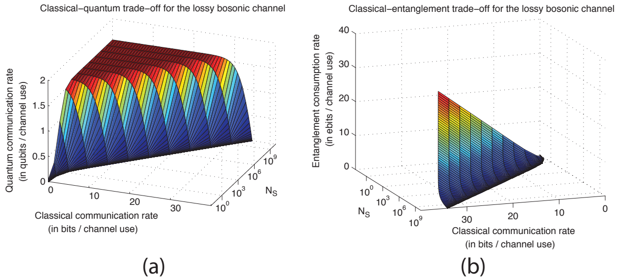
FIG. 3. (Color online) (a) The trade-off between classical and quantum communication for a lossy bosonic channel with transmissivity \eta = 3/4 as the mean input photon number N_S increases on a logarithmic scale from 0.01 to 10^{10} . The quantum capacity can never be larger than \ln(\eta) - \ln(1 - \eta) , but the classical capacity is unbounded as N_S \rightarrow \infty . Thus, the best option for a trade-off code is to abide by the rule of thumb given in the main text and dedicate only a small fraction \lambda \approx 50/[(1 - \eta) N_S] of the available photons to quantum resources. This ensures that the quantum data rate is near maximal while also maximizing the rate of classical communication. (b) The trade-off between entanglement-assisted and unassisted classical communication for the same lossy bosonic channel as N_S increases logarithmically from 0.01 to 10^{10} . Abiding by a similar rule of thumb and dedicating a fraction \lambda \approx 50/[(1 - \eta) N_S] of the available photons to shared entanglement ensures that the classical data rate is near maximal while minimizing the entanglement consumption rate. Observe that trade-off protocols operating at these near maximal data rates given by the rule of thumb consume about the same amount of entanglement for all of the trade-off curves depicted.
