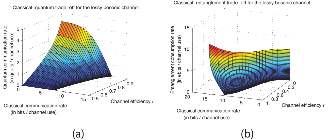
FIG. 2. (Color online) (a) The trade-off between classical and quantum communication for all \eta \in (1/2, 1) , with the result that trade-off coding always beats time-sharing by a significant margin. We assume that the mean input photon number N_S = 50/(1 - \eta) so that there are a sufficient number of photons to reach the quantum capacity of \ln(\eta) - \ln(1 - \eta) if the trade-off code dedicates all of the available photons to quantum communication. (b) The trade-off between entanglement-assisted and unassisted classical communication for all \eta \in (0, 1) , with the result that trade-off coding always beats time-sharing. For consistency with (a), we again assume that N_S = 50/(1 - \eta) .
