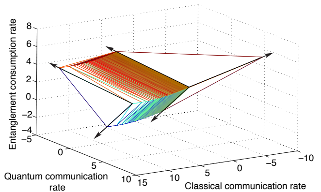
FIG. 1. (Color online) The full triple trade-off region for the lossy bosonic channel with transmissivity \eta = 3/4 and mean input photon number N_S = 100 . Units for classical communication, quantum communication, and entanglement consumption are bits per channel use, qubits per channel use, and ebits per channel use, respectively.
