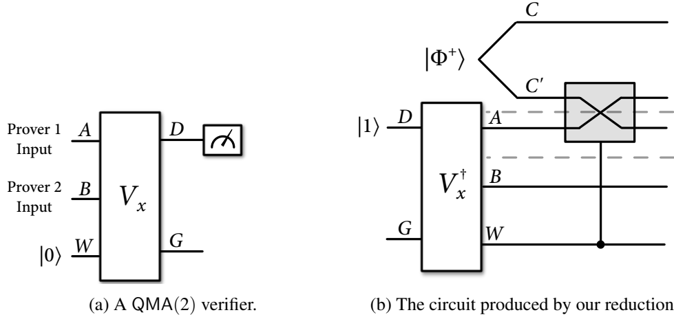
Figure 4: (a) A unitary verifier circuit V_x for an arbitrary verifier witnessing membership of L in \text{QMA}(2) on input x . (b) The circuit U produced by our reduction. Dashed lines indicate that the output registers are to be divided along the bipartite cut A : BCC'W .
