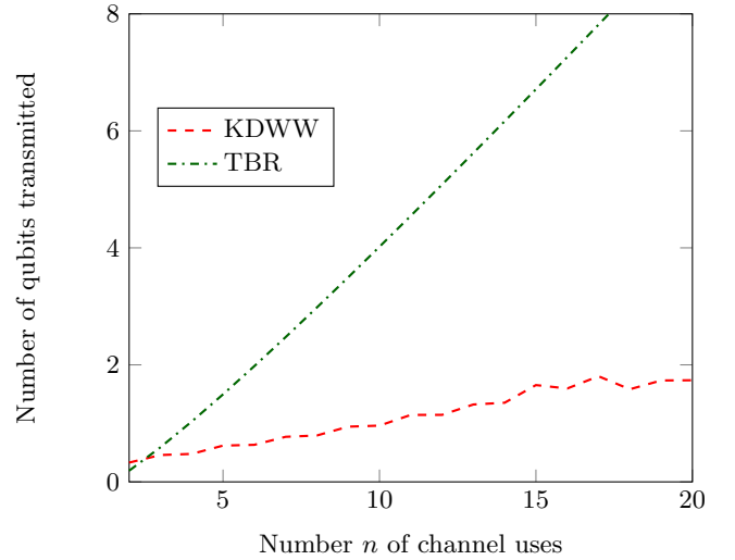
FIG. 6. Upper bounds on the number of qubits that can be reliably transmitted over an erasure channel with p = 0.35 , and \varepsilon = 0.05 . The red dashed line is the bound from Theorem 2. The green dash-dotted line is an upper bound from [TBR16].
