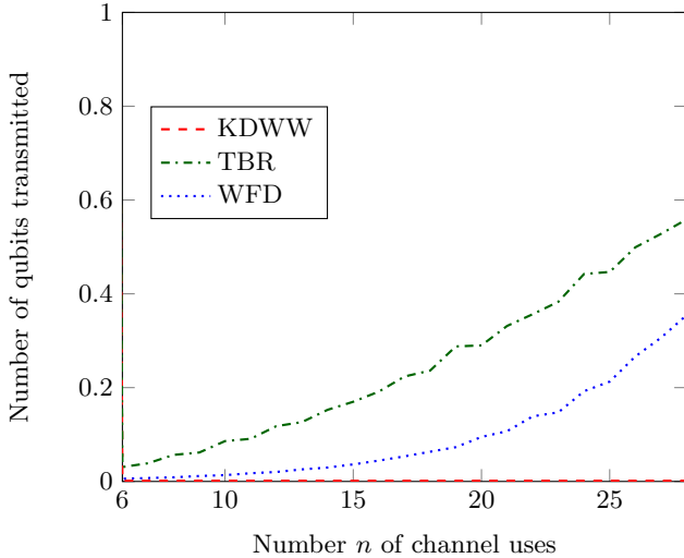
FIG. 5. Upper bounds on the number of qubits that can be reliably transmitted over a depolarizing channel with p = 0.25 , and \varepsilon = 5 \times 10^{-5} . The red dashed line is the bound from Theorem 2. The green dash-dotted and blue dotted lines are upper bounds from [TBR16] and [WFD19], respectively.
