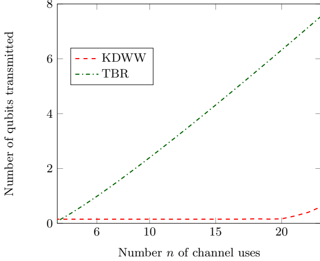
FIG. 7. Upper bounds on the number of qubits that can be reliably transmitted over an erasure channel with p = 0.49 , and \varepsilon = 0.05 . The red dashed line is the bound from Theorem 2. The green dash-dotted line is an upper bound from [TBR16].
