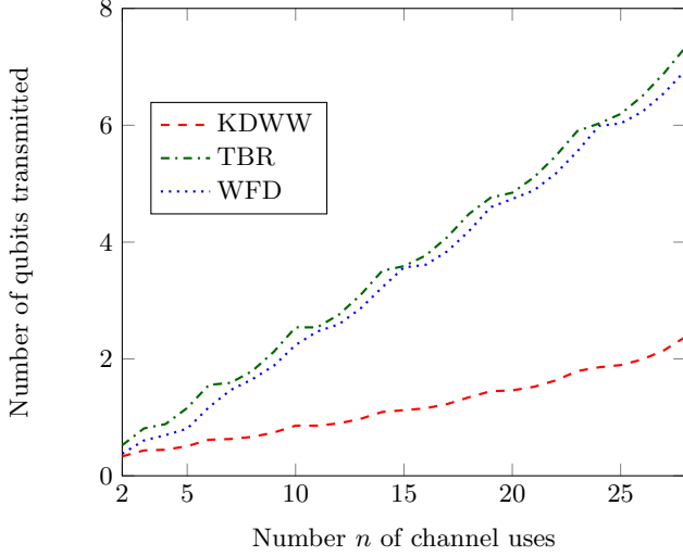
FIG. 4. Upper bounds on the number of qubits that can be reliably transmitted over a depolarizing channel with p = 0.1 , and \varepsilon = 0.05 . The red dashed line is the bound from Theorem 2. The green dash-dotted and blue dotted lines are upper bounds from [TBR16] and [WFD19], respectively.
