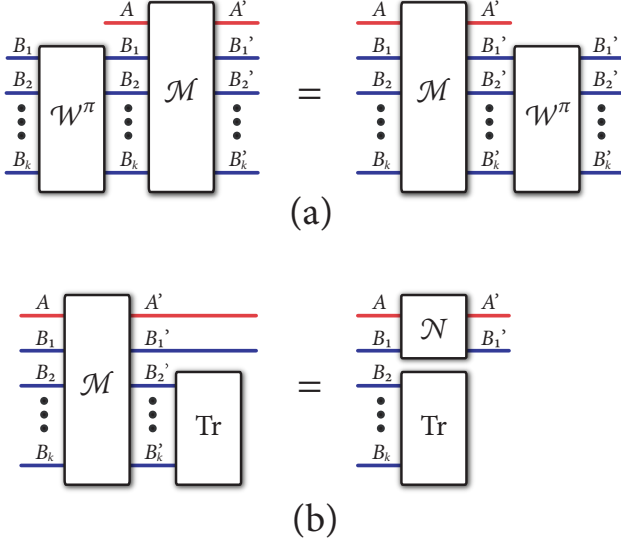
FIG. 1. A visual depiction of the conditions for the channel \mathcal{M}_{AB_1 \dots B_k \rightarrow A'B'_1 \dots B'_k} to be a k -extension of \mathcal{N}_{AB \rightarrow A'B'} . (a) The extension channel \mathcal{M}_{AB_1 \dots B_k \rightarrow A'B'_1 \dots B'_k} should be permutation covariant with respect to Bob's systems. (b) The extension channel \mathcal{M}_{AB_1 \dots B_k \rightarrow A'B'_1 \dots B'_k} should reduce to the original channel \mathcal{N}_{AB \rightarrow A'B'} when tracing out the output systems B'_2 \dots B'_k of \mathcal{M}_{AB_1 \dots B_k \rightarrow A'B'_1 \dots B'_k} .
