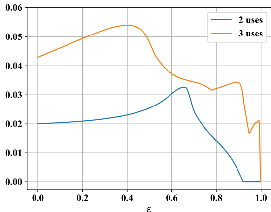
FIG. 4: Consider two GADCs with N = 0.2 and 0.3 respectively. They both have \gamma = 0.2 . We plot the difference between the distillable distinguishabilities, which is given by D_{\min}^{\epsilon}(\mathcal{N}^{(n)} \|\mathcal{M}^{(n)}) for the most general case and by D_{\min}^{\epsilon}(\mathcal{N}^{\otimes n} \|\mathcal{M}^{\otimes n}) for the case when a distinguisher is limited to a parallel strategy.
