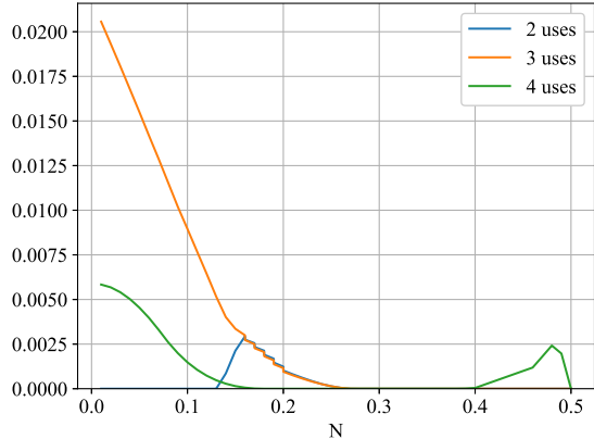
FIG. 3: Consider two GADCs with \gamma = 0.2 and 0.3 , respectively. We plot the difference between \frac{1}{2} \|\mathcal{N}^{(n)} - \mathcal{M}^{(n)}\|_{\diamond n} and \frac{1}{2} \|\mathcal{N}^{\otimes n} - \mathcal{M}^{\otimes n}\|_{\diamond} , where the strategies \mathcal{N}^{(n)} and \mathcal{M}^{(n)} each consist of n instances of the same channel. While varying the common parameter N , and allowing for different number of channel uses, we see that adaptive strategies offer an advantage in discrimination over parallel ones.
