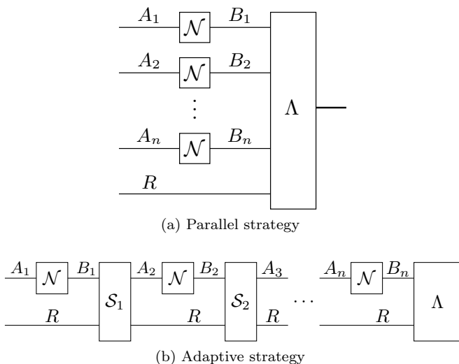
FIG. 2: Processing n uses of a channel \mathcal{N}_{A \rightarrow B} in (a) a parallel manner, and (b) an adaptive manner. In a parallel strategy, the input state to the n copies of the channel can be entangled, but the channels are all applied simultaneously. In an adaptive strategy, the channels are applied sequentially, with interleaving channels \mathcal{S}_1 through \mathcal{S}_{n-1} providing adaptive feedback. In a channel discrimination protocol, channels \mathcal{N}_{A \rightarrow B} and \mathcal{M}_{A \rightarrow B} are processed using a common apparatus and the final measurement results are used to decide the correct channel.
