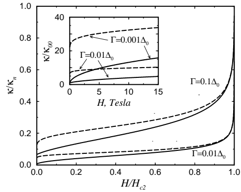
FIG. 1. Field dependence of the thermal conductivity at T = 0 for scattering in the unitarity (solid lines) and Born (dashed lines) limits. Inset: low field behavior, normalized by the universal value \kappa_{00} . H_{c2} = 150 T.
