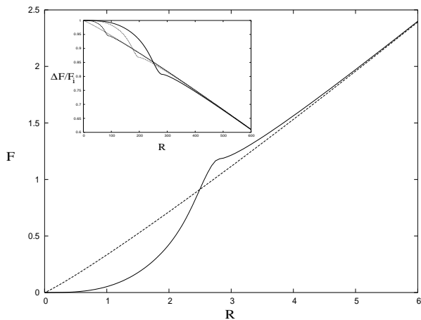
FIG. 2: Evolution of mass function with area radius for same parameters as in Fig.1. Loop quantum evolution (solid) leads to dissolution of all the mass of the collapsing shell. Dashed curve shows classical trajectory. Inset shows mass loss profile for j = 10^6 (outer), j = 5.0 \times 10^5 (middle) and j = 10^5 (inner).
