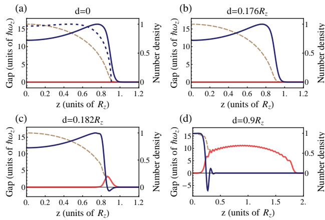
FIG. 3: (Color Online)(a-d) Spatial profile of the gap, total density, and magnetization in the z \geq 0 region (represented as in Fig. 1(b)) at d = 0, 0.176, 0.182, and 0.9R_z , respectively. In addition, in (a), the gap function obtained by BCS plus LDA is shown (dashed blue curve). In (b) and (c), the separations are just below and above the critical value d_c for appearance of the first node. Note the scale change on the z -axis in (d).
