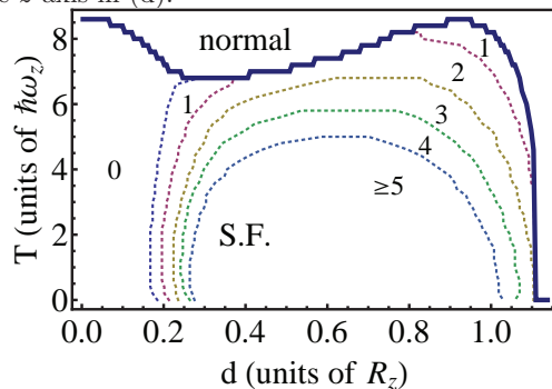
FIG. 4: (Color Online)Phase diagram as a function of separation and temperature ( N = 40, g/\hbar\omega_z R_z = 1 ). The solid line separates the normal phase and the superfluid phase. In the superfluid phase, the dashed lines separate regions of the gap functions with different number of nodes.
