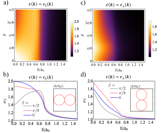
FIG. 2. Conductance of a lateral heterojunction with a chiral parent SC. Panels a) and b) (panels c) and d)) are for the TI-SC interface described by \mathbf{c}_{\parallel}(\mathbf{k}) ( \mathbf{c}_{\perp}(\mathbf{k}) ), see text. Top row shows the color map as a function of the boundary parameter \beta in Eq. (6), bottom row shows \sigma_T for select values of \beta . The insets give the shape of the induced superconducting gap at the interface.
