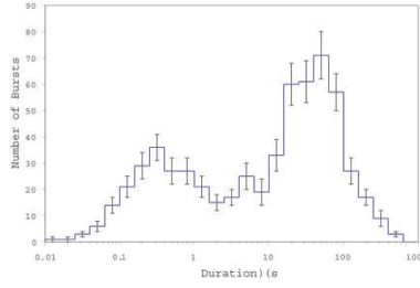
Fig. 1.— Burst duration versus number for GRBs detected by BATSE. The two peaks occur at \sim 0.3 second and \sim 30 seconds (based on Meegan et al. (1996)).
