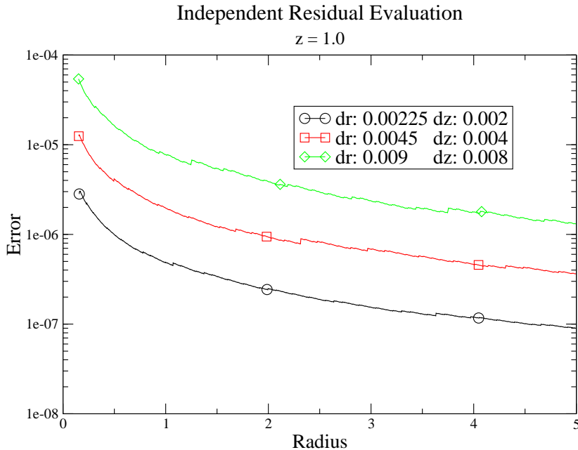
FIG. 1: The unscathed error for a uniform black string along the radius at z = 1 at three resolutions. For the highest resolution at r = 0.01 , the error scaled by \bar{\rho} + 1 was 1.3 \times 10^{-5} ; \bar{\rho} was 3.48 \times 10^5 .
