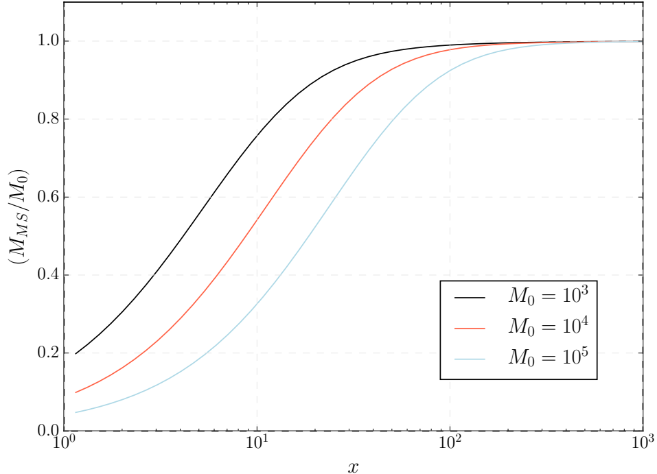
FIG. 6: Misner–Sharpe mass (normalized to the corresponding mass M_0 ) for different values of M_0 .
