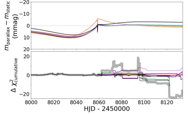
Figure 3. (Top) Difference of best-fit model magnitudes between the parallax and static models for individual data sets, where the color codes are the same as in Figure 1. (Bottom) Difference of cumulative \chi^2 between the parallax and static models for individual data sets (thin colored lines) and all data sets (thick gray line), where negative means that the parallax model is preferred. The color codes are the same as in Figure 1.
