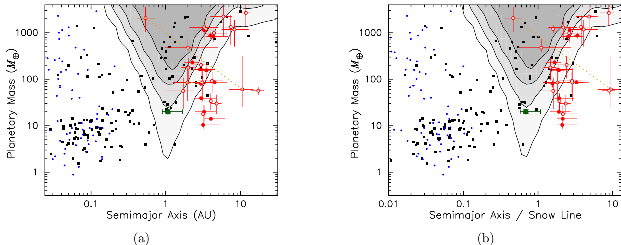
Figure 11. (a) Distribution of known exoplanets in the planetary mass and semimajor axis planes for the host stars having a mass of 0.4\text{--}0.8 M_{\odot} . Data are collected mainly from http://exoplanet.eu . Black squares, blue circles, and red circles indicate the planets observed by radial velocity, transit, and microlensing, respectively. The filled and open circles of microlensing show the planets with and without direct mass constraint, respectively. Two degenerated solutions are connected by a dotted line, if applicable. Kojima-1Lb is depicted as a green circle. The contours show the planet detection efficiencies for Kojima-1 of 90%, 70%, 40%, and 10% (top to bottom). (b) Same as (a), but the x -axis is converted to the semimajor axis normalized by the snow-line location estimated by a_{\text{snow}} = 2.7 \times M_{*}/M_{\odot} au.
