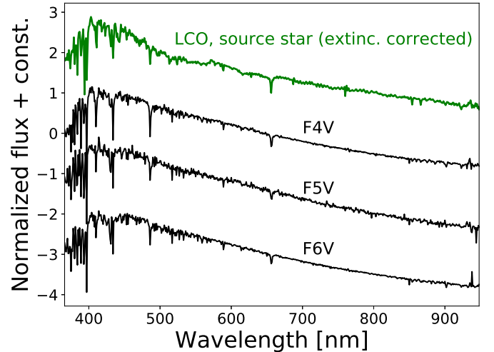
Figure 6. Low-resolution spectrum of the source star extracted and extinction-corrected from the LCO spectra (green), along with empirical spectral templates of F4V, F5V, and F6V stars from Kesseli et al. (2017) (black, top to bottom).
