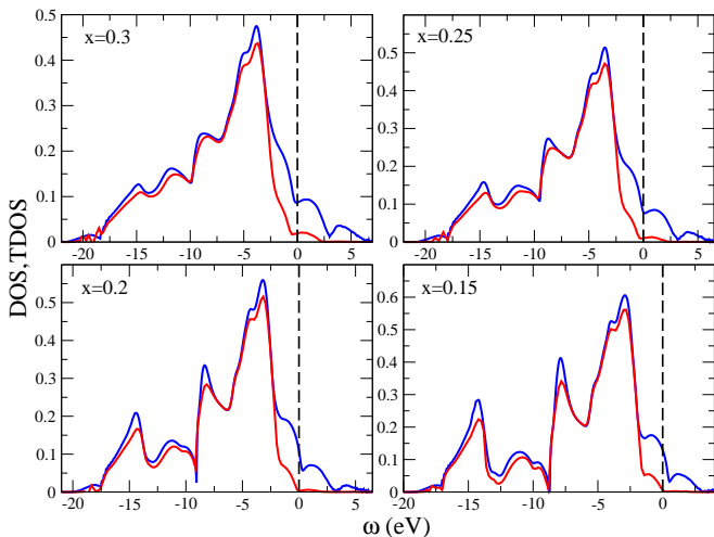
FIG. 5. DOS (blue) and typical DOS (red) of \text{Ga}_{1-x}\text{Mn}_x\text{N} for higher Mn concentrations: x=0.15, 0.2, 0.25, 0.3 , with N_c=32 , showing a transition to the metallic state happens around x = 0.25 . The chemical potential is set to be zero and denoted as the dash line.
