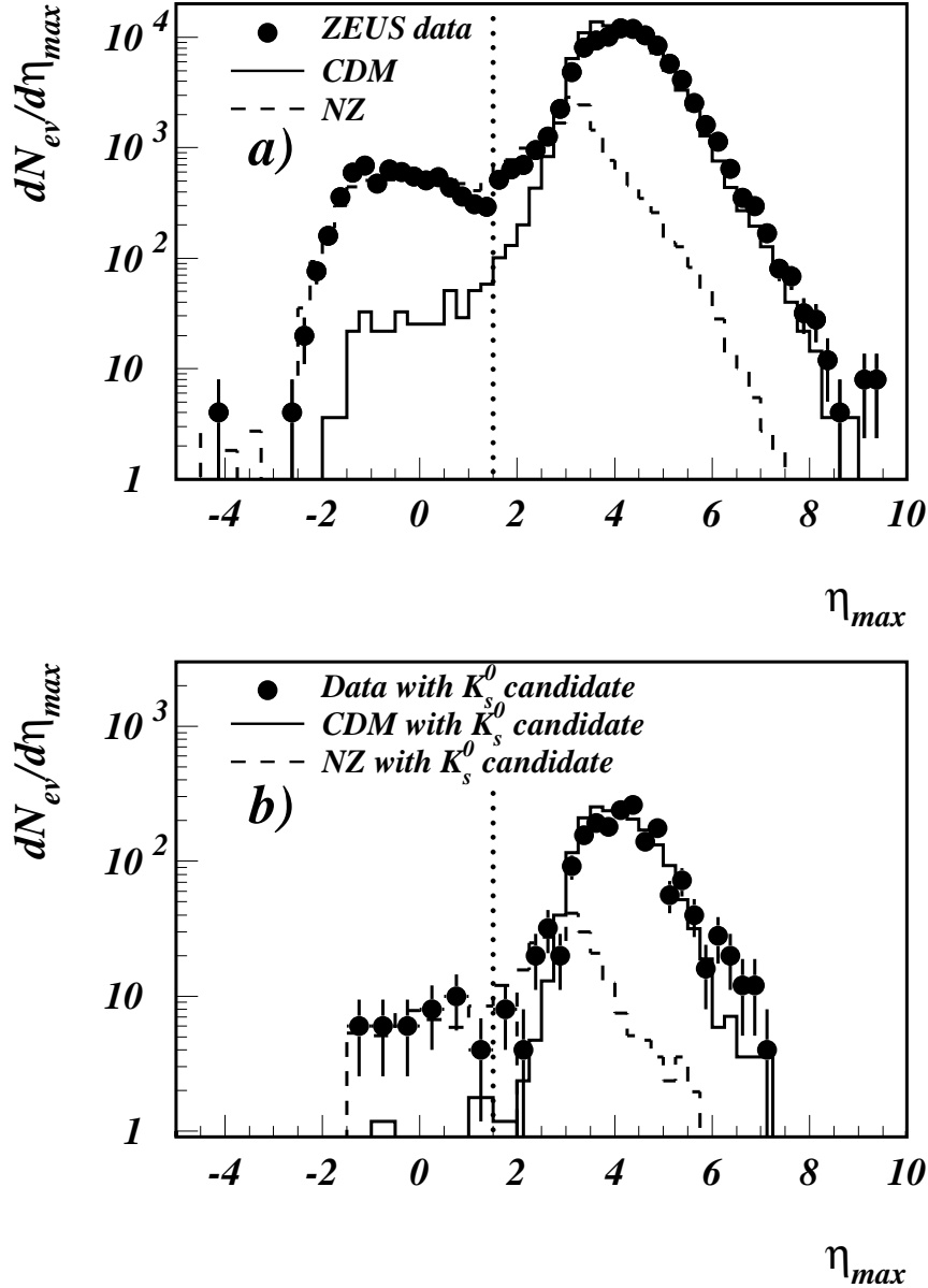
Figure 7: a) \eta_{max} distribution for all selected events, for one of the non-diffractive Monte Carlo samples (CDM) and for one of the diffractive Monte Carlo samples (NZ). The relative fractions of CDM (88%) and NZ(12%) events are chosen so that their sum reproduces the data distribution best. b) \eta_{max} distribution of events with a K_s^0 candidate in the signal region of the M_{\pi\pi} distribution. The predictions of the CDM model and of the NZ model are overlaid. The dotted line corresponds to \eta_{max} = 1.5 .
