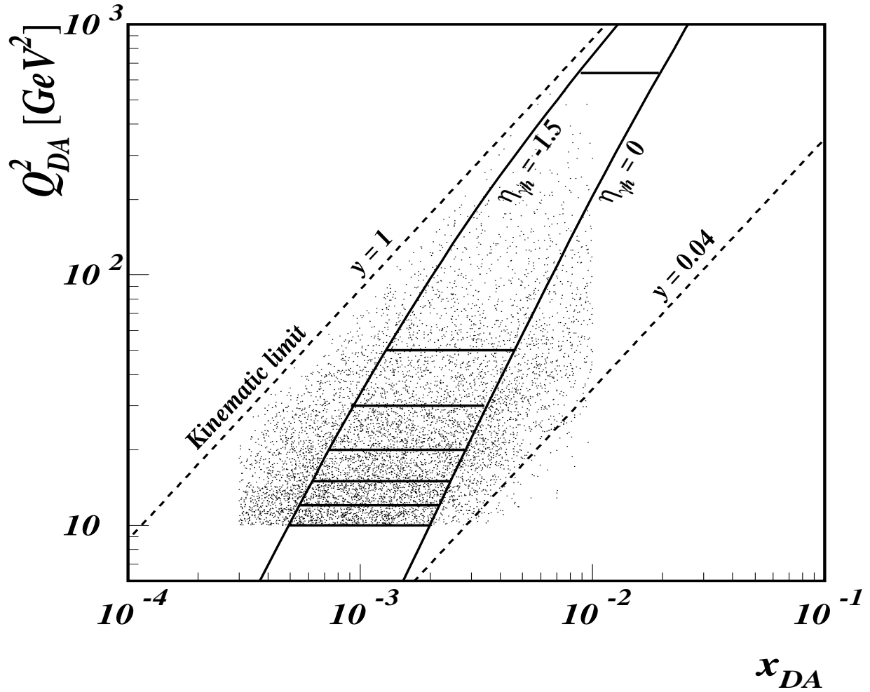
Figure 5: The (x, Q^2) plane with lines of constant \eta_{\gamma_h} . For the determination of the Q^2 dependence of the K^0 multiplicity only events with -1.5 < \eta_{\gamma_h} < 0 are accepted. The horizontal lines correspond to the Q^2 bins chosen.
