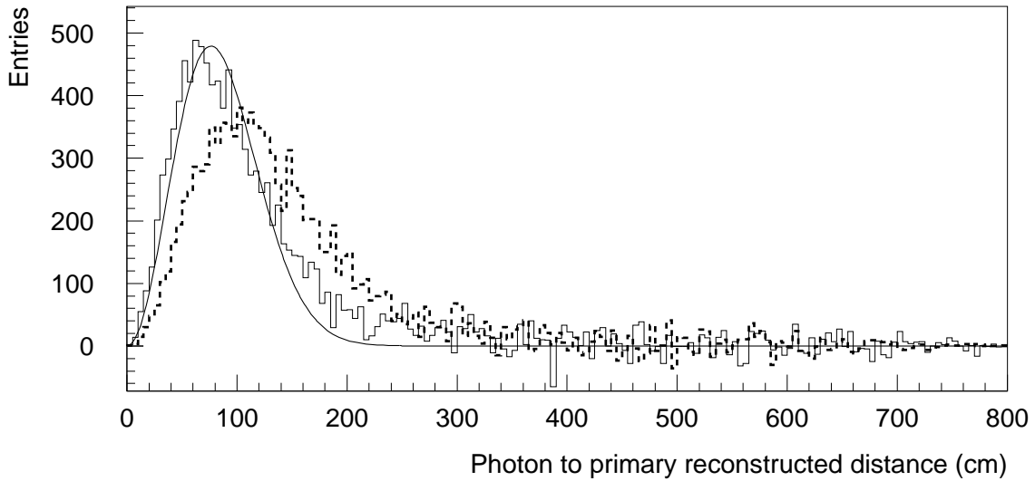
FIG. 30. Photon to primary reconstructed distance for the old (dashed histogram) and new reconstruction algorithms (solid histogram) for correlated photons. The average distance is decreased from 76 cm to 54 cm. The superimposed fit is to f(dr) = C dr^2 \exp[-dr^2/(2\sigma^2)] .
