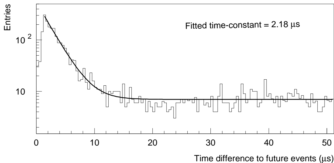
FIG. 3. Time difference distribution to events subsequent to all primary events for the initial DIF data after standard PID, veto shield hit multiplicity and fiducial volume cuts.
