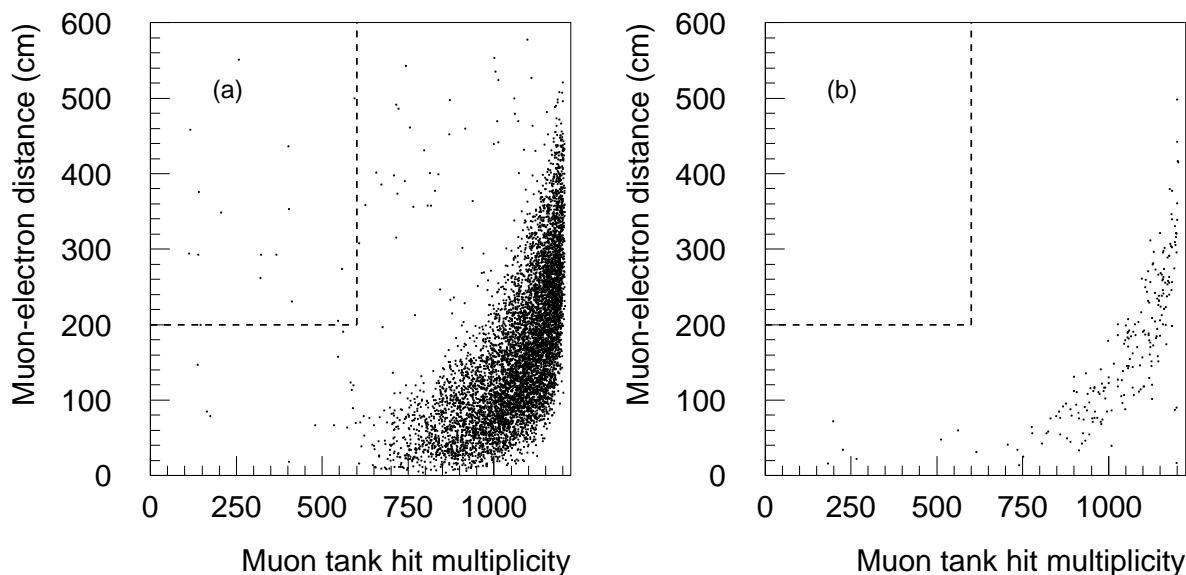
FIG. 4. Reconstructed distance distribution between Michel electron and parent stopped cosmic-ray muon, versus muon tank hit multiplicity. Figure (a) is for muons with a veto shield hit multiplicity \geq 6 and (b) is for muons with a veto shield hit multiplicity < 6 . The regions in the upper left corners, delimited by the dashed lines, are the regions allowed by this selection (see text).
