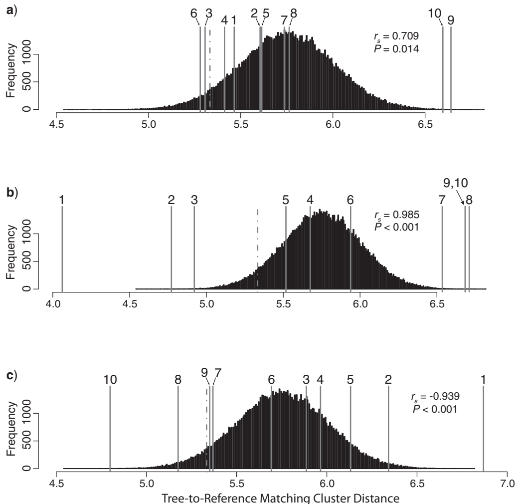
FIGURE 3. Mean matching cluster distance between amniote UCE ML trees and the reference topology for each filtered decile. A) Mean matching cluster distance to the reference topology within each decile ranked by likelihood ratio test statistics. B) Mean matching cluster distance to the reference topology within each decile ranked by rate of evolution. The null distribution was estimated by resampling 114 (10%) ML amniote UCE trees and recalculating the mean matching split distance to the reference topology 100,000 times. Numbers separated by commas indicate means that are identical. r_s is Spearman's rank correlation coefficient between decile indices and the ranked mean distances to the reference topology.
