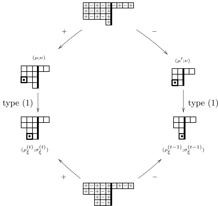
Figure 2: Simultaneous degeneration of subordinate bipartitions
