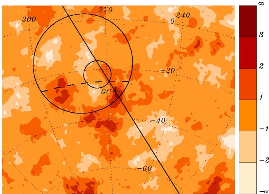
Fig. 1. Map of CR overdensity significances near the GC region on top-hat windows of 5^\circ radius. The GC location is indicated with a cross, lying along the galactic plane (solid line). Also the regions where the AGASA experiment found their largest excess as well as the region of the SUGAR excess are indicated.
