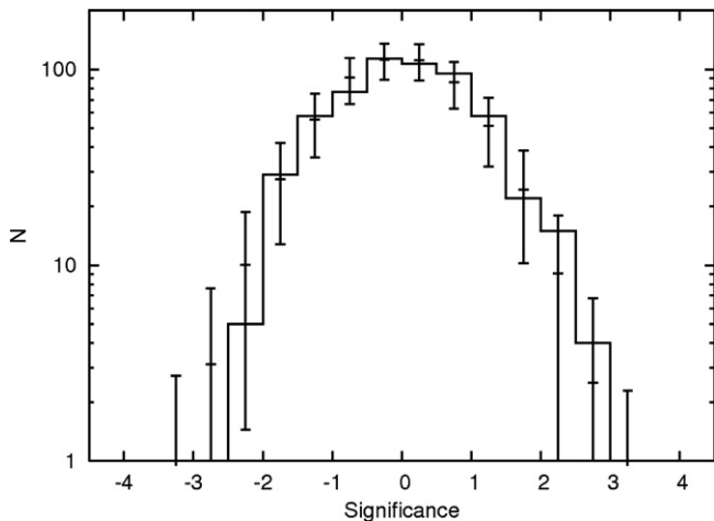
Fig. 2. Histogram of overdensities on 5^\circ radius windows and for 10^{17.9} \text{ eV} < E < 10^{18.5} \text{ eV} , together with isotropic expectations (average and 2\sigma bounds). Overdensities are computed on a grid of 3^\circ spacing for the patch of the sky depicted in Fig. 1.
