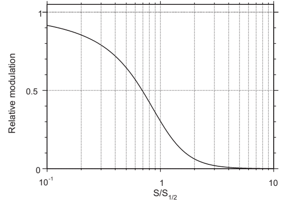
Fig. 2. Relative modulation of the rates above a given corrected signal size due to the variations of the detection efficiency under changes of atmospheric conditions, relatively to the factor modulating the rate of events above the corresponding uncorrected signal size in units of S_{1/2} .
