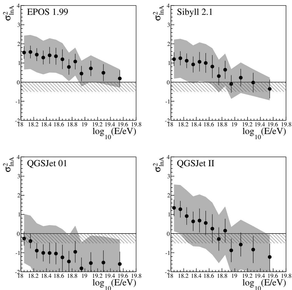
Figure 5. \sigma_{\ln A}^2 as a function of \log_{10}(E/eV) obtained from Auger data [22] are shown as full circles for different hadronic interaction models. Error bars show statistical errors. The shaded area refers to systematic uncertainties as in figure 4. The lower limit of allowed \sigma_{\ln A}^2 is shown by the exclusion line. The upper limit (4.05) is just above the maximum of the vertical axis.
