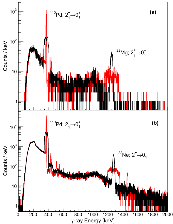
Fig. 1. Doppler-corrected \gamma -ray spectra for (a) ^{22}\text{Mg} impinged on a ^{110}\text{Pd} target at 92.4 MeV, (b) ^{22}\text{Ne} impinged on a ^{110}\text{Pd} target at 54.8 MeV. Doppler-corrected for ^{22}\text{Mg} and ^{22}\text{Ne} (black) and ^{110}\text{Pd} (red). (For interpretation of the colors in the figure(s), the reader is referred to the web version of this article.)
