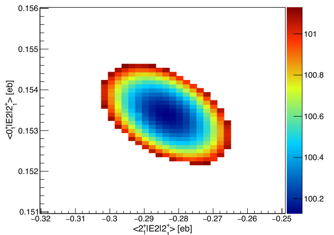
Fig. 4. \chi^2 surface at the \chi_{\text{min}}^2 + 1 ( 1\sigma ) limit for the \langle 0_1^+ | E2 | 2_1^+ \rangle and \langle 2_1^+ | E2 | 2_1^+ \rangle matrix elements in ^{22}\text{Ne} .
