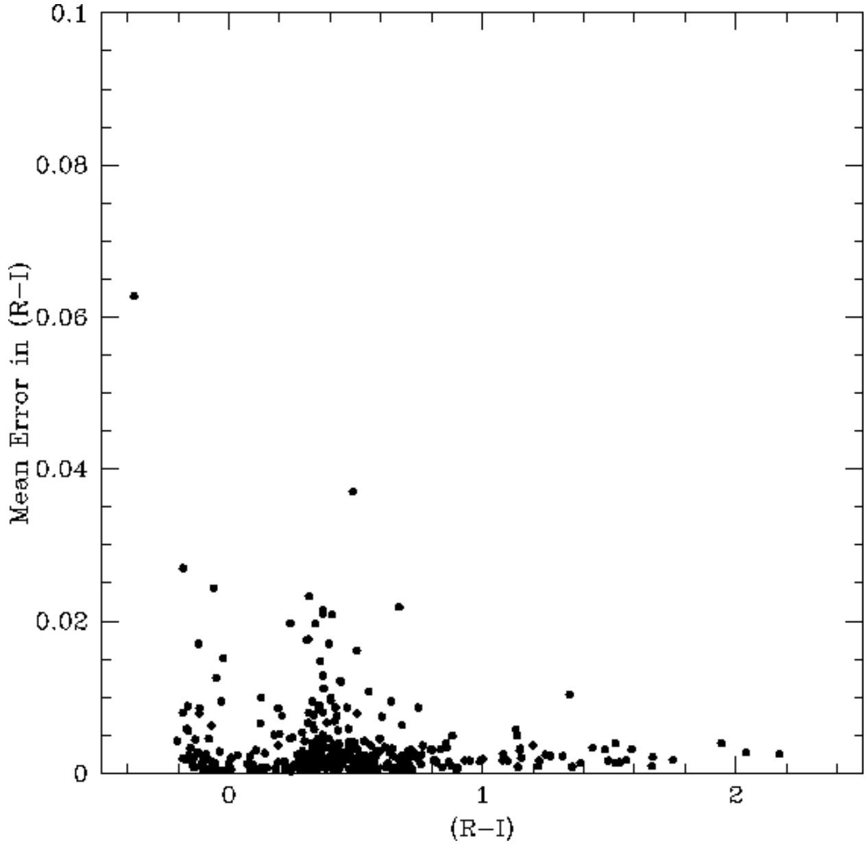
Fig. 8.— Mean error of the mean of a single observation in (R - I) for the standard stars as a function of (R - I) .
