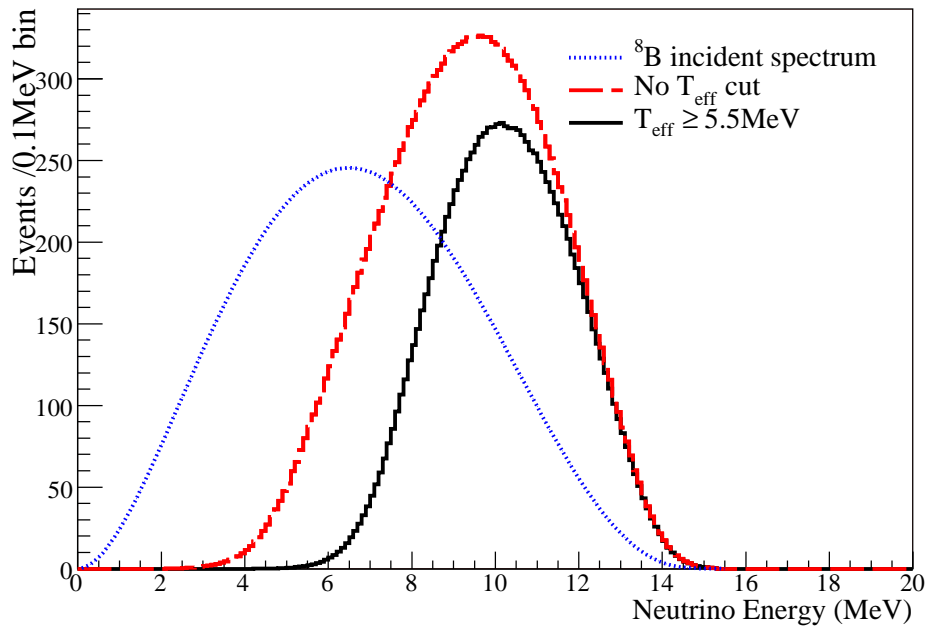
Fig. 1.— Monte Carlo simulation of the {}^8\text{B} solar neutrino energy spectrum. The dotted curve is the incident spectrum of neutrinos from the Sun with an arbitrary normalization, the dashed curve shows the spectrum of those detected by the CC reaction before any cut on the kinetic energy of the created electron, and the solid curve shows the spectrum of neutrinos seen after the application of the kinetic energy threshold for Phase II.
