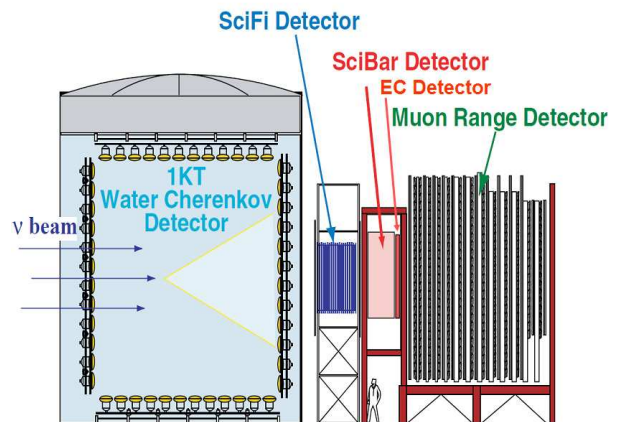
FIG. 2. Schematic view of the near neutrino detector.
