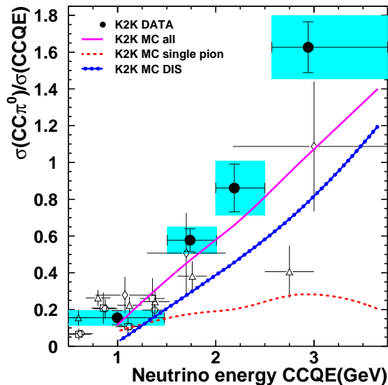
FIG. 11. CC\pi^0 to CCQE cross section ratio as a function of neutrino energy. The result of this analysis ( \bullet ) is compared with our standard MC expectation and past experimental results. The previous experimental data are: ( \circ )ANL82[11], ( \square )ANL[33], ( \triangle )BNL86[12], ( \diamond )ANL83+BNL86[14][12](see text for details).
