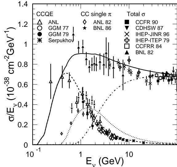
FIG. 4. Charged-current total cross section divided by the neutrino energy E_{\nu} for neutrino-nucleon charged-current interactions[32]. The solid line shows the calculated total cross section. The dashed, dotted and dash-dotted lines show the calculated quasi-elastic, single pion and deep inelastic scattering, respectively. The data points are taken from the following experiments: ( \Delta ) ANL[33], ( \circ ) GGM77[34], ( \bullet ) GGM79 (a)[35], (b)[36], ( * ) Serpukhov[37], ( \diamond ) ANL82[11], ( * ) BNL86[12], ( \blacksquare ) CCFR90[38], ( \blacktriangledown ) CDHSW87[39], ( \times ) IHEP-JINR96[40], ( + ) IHEP-ITEP79[41], ( \square ) CCFRR84[42], and ( \blacktriangle ) BNL82[43].
