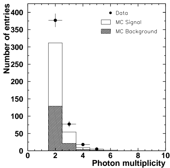
FIG. 6. Photon multiplicity of CC\pi^0 candidate events
