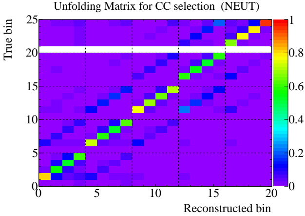
FIG. 10. The unfolding matrix obtained with the NEUT MC simulation. The white line corresponds to backward-going muons in the highest energy bin, for which our MC prediction is zero events. The x-axis and y-axis bin numbering is defined in Table X and Table XI respectively.
