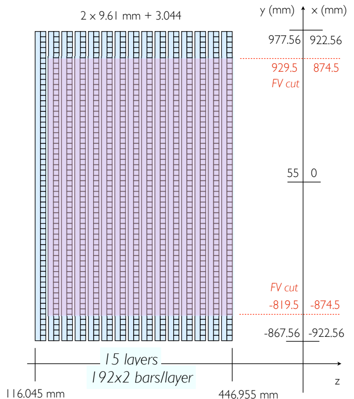
FIG. 4. Schematic view of FGD1 and its fiducial volume (FV) drawn in red. In the y-coordinate, the detector is displaced 55 mm upwards relative to the center of the ND280 coordinate system, which is centered in the magnet.
