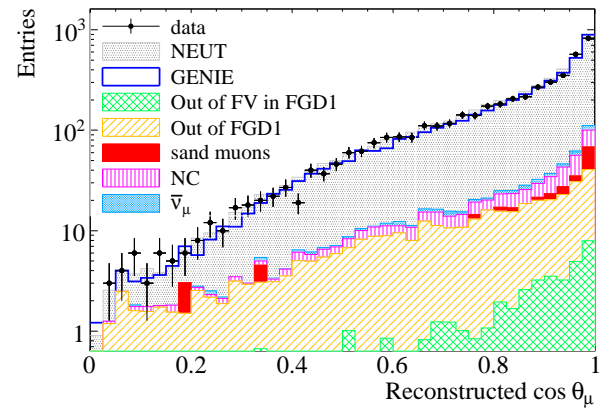
FIG. 9. The muon momentum and angle distribution for the selected events in the data and MC. The GENIE prediction is shown by the solid blue line, while the backgrounds and signal as derived from NEUT are shown in filled colors.
