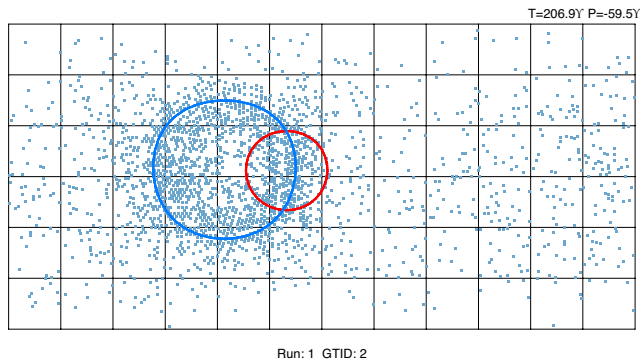
FIG. 7. Visual display of the small-ring pathology of a simulated e^- event. The blue ring is the primary ring, ring with the best reconstruction (i.e. minimum of -2 \ln \lambda_\alpha in Eqn. 7), while the red is the secondary ring. This secondary ring is a MRF flaw in handling low statistics of triggered PMTs if the local vertex ( x'_{\text{rec}} \hat{u}_{\text{rec}} ) is near the acrylic vessel. This pathology appears when the reconstruction of the local vertex from the origin is x'_{\text{rec}} > 350 cm along the track.
