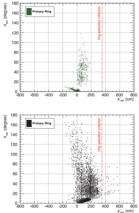
FIG. 6. Reconstruction of \pi^+ simulated at the origin of the detector using a non-showering (top) and showering (bottom) expectation, highlighting the complexity of single pion reconstruction. x'_{rec}\hat{u}_{rec} is the reconstructed vertex position and \theta_{rec} is the angle of the reconstructed track with respect to the original true track. Visual cross-verification of these events shows good ring recognition except for rings with x'_{rec} > 350 cm. This is used as a ring selection criterion.
