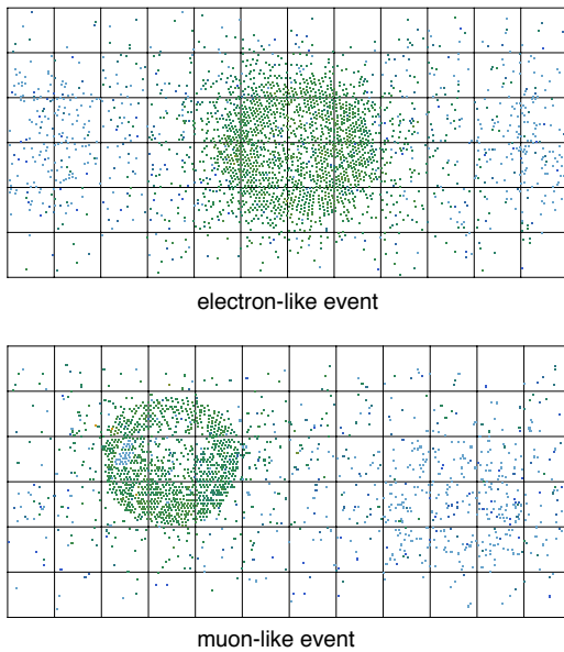
FIG. 3. Simulated Cherenkov electron ring (top) demonstrating the showering effect and muon ring (bottom) demonstrating the absence of the showering effect. Both particles were generated with 600 MeV of kinetic energy and placed at the center of the detector; the resulting PMT hit pattern is projected in (\cos \theta_{\text{PMT}}, \phi_{\text{PMT}}) space. The colors shown represent the time the PMT has been hit, where green points represent PMTs that were hit first and blue points are PMTs that were hit at a later time.
