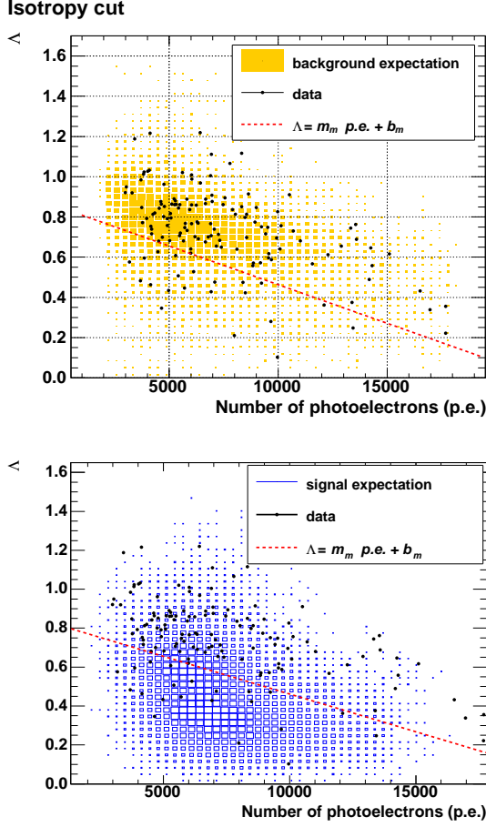
FIG. 9. Scatter plot of the \Lambda parameter (Eqn. 8) and the number of photoelectrons for the background and signal expectation of multiple-ring events. The red line denotes the isotropy cut applied to the data set to isolate signal events from background events (detailed in Sec. VI).
