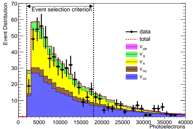
FIG. 2. Comparison between the data and the simulated SNO detector response to contained atmospheric neutrinos using the corrected Bartol fluxes. The channel composition is defined in Eqn. 5. Since n-\bar{n} events are constrained in an energy window between 2,000 and 18,000 photoelectrons (Figure 1), only atmospheric contained events in this energy range are selected. A selection criterion requiring that signal is present in at least 2,000 photomultiplier tubes in an event is applied.
