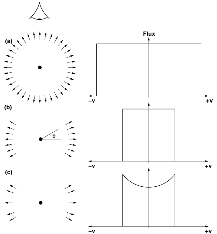
Fig. 13. Illustrative optically thin profiles for different outflow geometries. The viewing angle is taken to be from the top of the page, i.e. pole-on. a) A spherically symmetric outflow produces a square profile extending to \pm V_{\text{term}} . b) An equatorial section of a spherical outflow also produces a square profile (when viewed pole-on), but narrower, extending to \pm V_{\text{term}} \sin \theta . c) If the outflow is non uniform, with less emission closer to the equatorial plane, then a central depression is created, because there is less low velocity emission.
