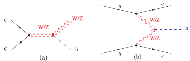
FIG. 1 (color online). The dominant production diagrams for the benchmark fermiophobic Higgs boson model: associated production with a vector boson (a), and vector boson fusion (b).
