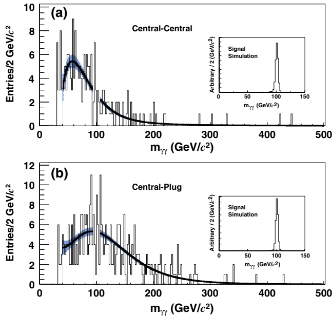
FIG. 2 (color online). The invariant mass distribution of central-central (a) and central-plug (b) photon pairs after the requirement of p_T^{\gamma\gamma} > 75 GeV/ c , shown with the fit to the data for the hypothesis of a m_h of 100 GeV/ c^2 . The gap in the fit centered at 100 GeV/ c^2 represents the signal region for this mass point that was excluded from the fit. The error bands show the statistical uncertainty in the fit. The expected shape of the signal from simulation is shown in the insets.
