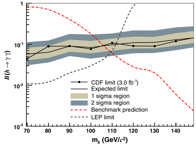
FIG. 3 (color online). The 95% C.L. upper limit on the branching fraction for the fermiophobic Higgs boson decay to diphotons, as a function of m_h . The shaded regions represent the one and two sigma probability of fluctuations of the observed limit away from the expected limit based on the distribution of possible experimental outcomes. For reference, the 95% C.L. limits from LEP are also included.
