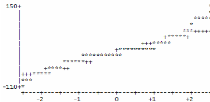
Figure 8. The normal probability plot of the residuals of travel empty, grapple time, travel loaded, and un-grapple time.
