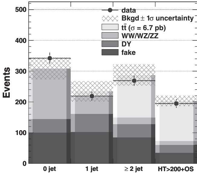
FIG. 9. Dilepton candidate events (black point) by jet multiplicity. The stacked histogram represents the background contribution and the t\bar{t} contribution for an assumed \sigma_{t\bar{t}} = 6.7 pb. The hatched area is the uncertainty in the total background estimate.
