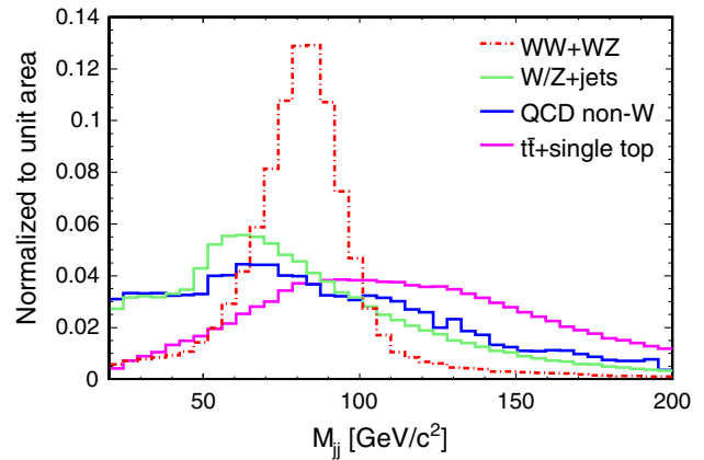
FIG. 10 (color online). Shape of M_{jj} templates for signal and background processes normalized to unit area.
