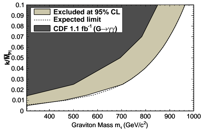
FIG. 4: The 95% C.L. excluded region in the plane of k/\overline{M}_{Pl} and graviton mass from 5.4 fb -1 of integrated luminosity compared with the expected limit and the previously published exclusion contour [4].
