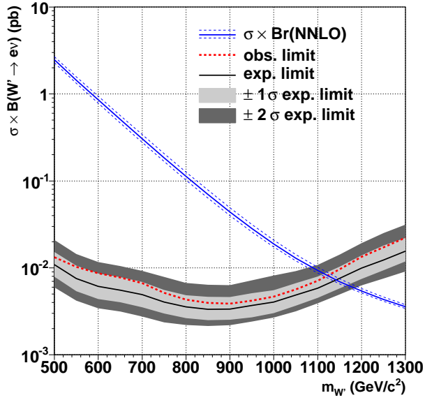
FIG. 3: The 95 % CL limits on cross section times branching fraction as a function of W' boson mass and the expected limits from the simulated experiments with background only. The black solid lines represent median expected, the shaded bands indicate the \pm 1\sigma and \pm 2\sigma intervals on the expected limits. The region above the red dashed line (observed limit) is excluded at the 95 % CL. The cross section times branching fraction assuming the manifest LR symmetric model, \sigma \cdot \mathcal{B}(W' \rightarrow e\nu)_{LR} , is shown along with its uncertainty. The intercept of the cross section limit curve and the lower bound of the theoretical cross section yields m_{W'} > 1.12 \text{ TeV}/c^2 at the 95 % CL.
