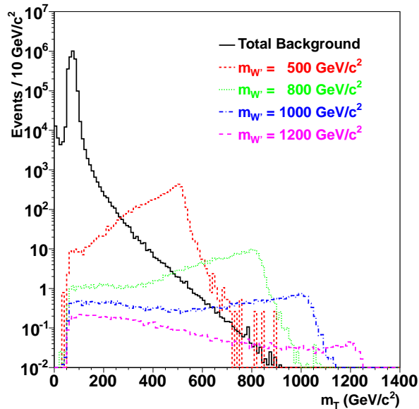
FIG. 1: The transverse mass distributions for W' \rightarrow e\nu signal events generated using PYTHIA with total background expectation.
