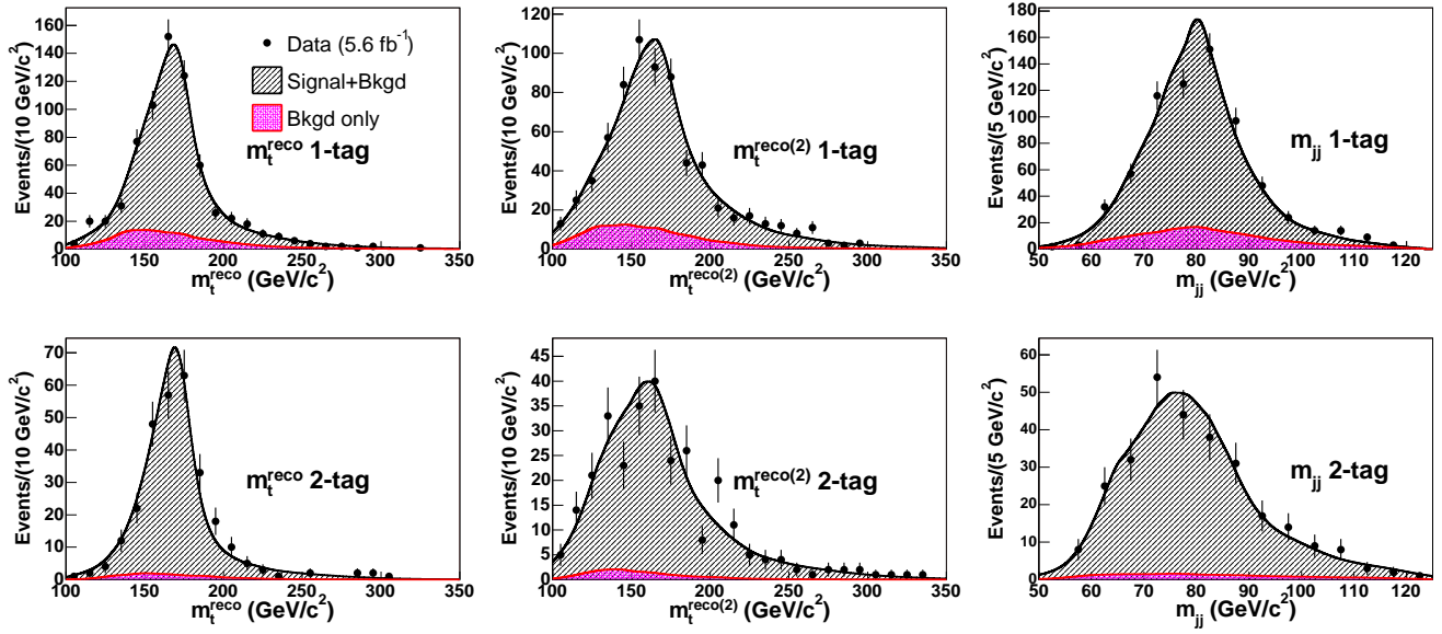
FIG. 1: Distributions of the three variables used to measure M_{\text{top}} in the lepton+jets channel, showing 1-tag and 2-tag samples separately. The data are overlaid with the predictions from the KDE probability distributions using M_{\text{top}} = 172.0 \text{ GeV}/c^2 and the full background model.
