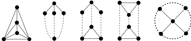
Figure 1.4: Graphs K_5 \setminus e , H_0 , H_1 , H_2 , and H_3 (wheel), where a dotted indicates a chordless path containing one or more edges [3].
