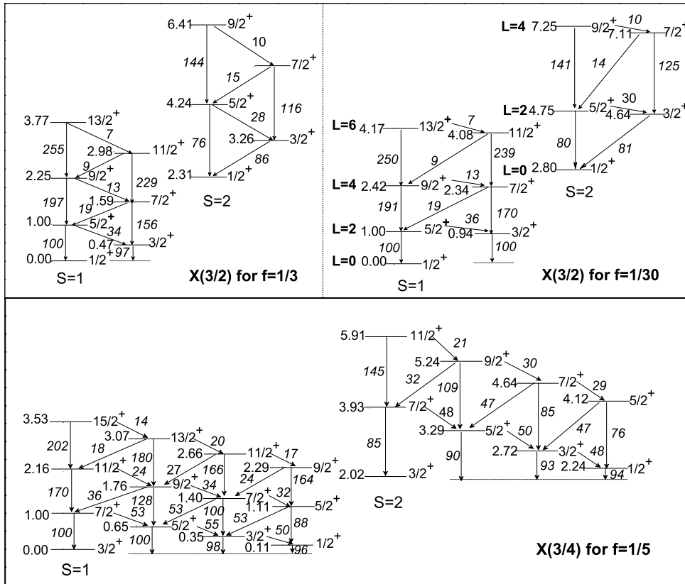
FIG. 1: The spectrum of the X(3/2) model with f = 1/3 and f = 1/30 corresponding to the case of the X(3) even-even core coupled to an s_{1/2} , and the X(3/4) model with f = 1/5 corresponding to the case of the core coupled to a d_{3/2} particle. For p_{1/2} or p_{3/2} case, all parities should be reversed. In our calculation, the parameter b in Eq (3) has been taken as zero, and all energy levels are normalized to the energy of the first (j+2)_1^+ excited state and the B(E2) transition values are normalized to that of the B(E2; (j+2)_1^+ \rightarrow j_1^+) .
