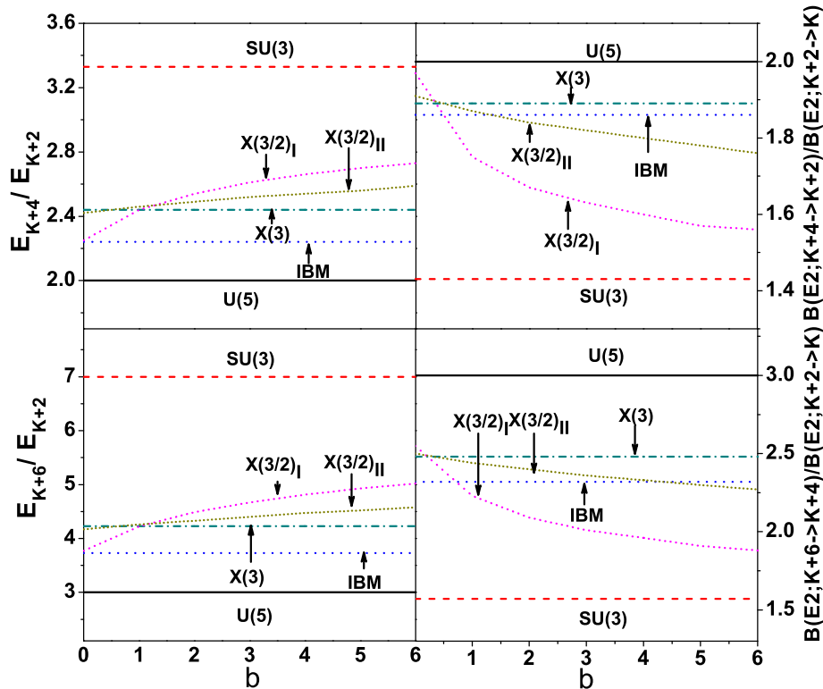
FIG. 2: Typical energy ratios and B(E2) ratios as functions of the parameter b in different models. For odd-A systems, X(3/2)_I and X(3/2)_{II} curves represent the results obtained from the X(3/2) model for the strong coupling case ( f = 1/3 ), and the weak coupling case ( f = 1/30 ), respectively. For even-even systems, X(3) curves denotes the results obtained from the X(3) model [5], while U(5), SU(3), and IBM curves represent the results calculated from the U(5) limit, SU(3) limit, and the critical point of U(5)-SU(3) phase transition in the interaction boson model with N = 10 , respectively, where the results characterized by U(5), SU(3), and IBM are calculated with the Hamiltonian H = c[(1 - \xi)n_d - \frac{\xi}{4N}(Q^x \cdot Q^x)] used in [15]. In addition, K = 0 for even-even systems and K = 1/2 for odd-A systems.
