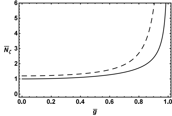
FIG. 2: (Color online) The ground-state expectation value of total number of bosons \bar{N}_{\zeta=1} (solid curve) and that of the first excited intruder 0_1^+ state \bar{N}_{\zeta=2} (dashed curve) defined by (34) and (35), respectively, as functions of the mixing parameter \bar{g} = g/\epsilon_d , where N = 10 and \bar{\Delta} = \Delta/\epsilon_d = 1 is taken in the plot.
