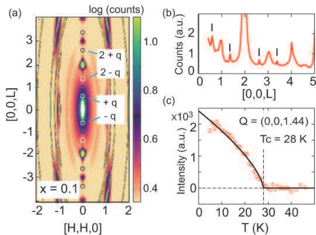
FIG. 7: (a) Neutron diffraction measurements on \text{Sr}(\text{Co}_{0.9}\text{Ni}_{0.1})_2\text{As}_2 in the [H, H, L] plane 24 . (b) One-dimensional cut along the [0, 0, L] direction in (a). The intensities at (0, 0, L) with L = \text{odd} number are due to double scattering 34 . (c) Temperature dependence of the magnetic peak at Q = (0, 0, 1.44) .
