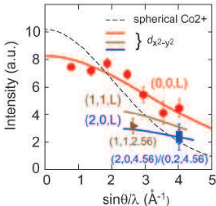
FIG. 8: Integrated intensity of magnetic Bragg peaks. The dashed curve is the magnetic form factor of \text{Co}^{2+} using a spherical approximation. The solid curves are magnetic form factors for the d_{x^2-y^2} orbital multiplied with a polarization factor along different measured directions for a helical order. Red, brown and blue are along the [0, 0, L] , [1, 1, L] , and [2, 0, L]/[0, 2, L] directions, respectively.
