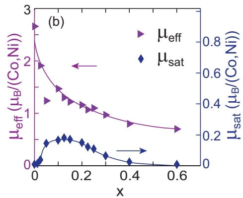
FIG. 4: Effective magnetic moment, \mu_{eff} , by fits of the C-W law to the magnetic susceptibility above T_c , and saturated magnetic moment, \mu_{sat} , vs. x . The large ratio of \mu_{eff}/\mu_{sat} reflects the itinerant nature of magnetism.
