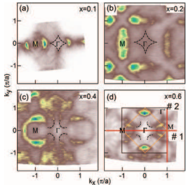
FIG. 9: Plot of the ARPES intensity at E_F of \text{Sr}(\text{Co}_{1-x}\text{Ni}_x)_2\text{As}_2 with x = 0.1, 0.2, 0.4, \text{ and } 0.6 . A complex structure of Fermi surfaces is observed and the topology changes dramatically from x=0.1 to x=0.6 due to the existence of flat band dispersion. The dashed lines curves are guide to the eye.
