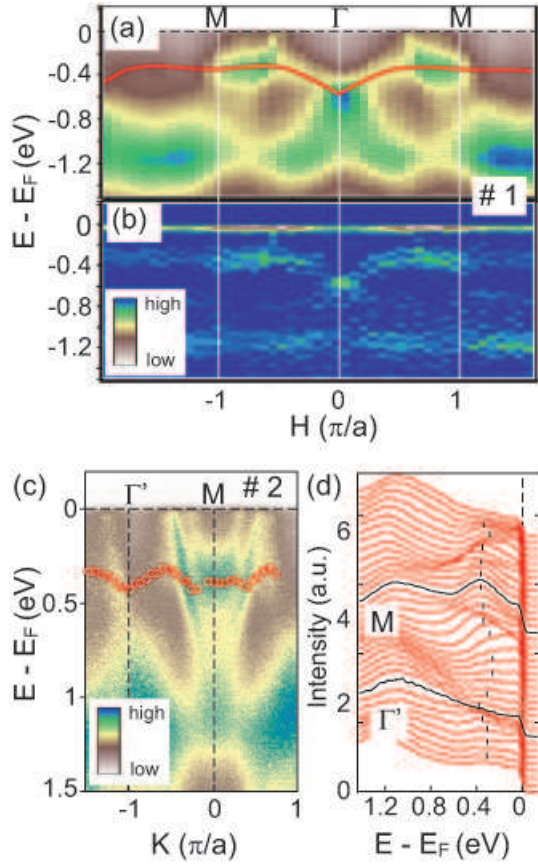
FIG. 11: (a) and (b) ARPES Intensity plot and its second derivative along the cut #1 direction as shown in Fig. 9 (d). (c) and (d) ARPES spectra along the cut #2 direction and its corresponding Energy distribution curve (EDC).
