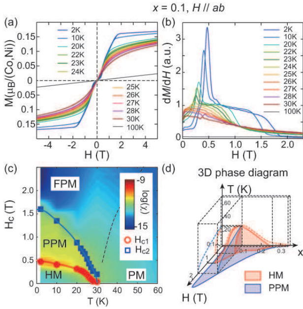
FIG. 5: (a),(b) M_{ab} and dM_{ab}/dH vs. H at temperatures identified in the figures. (c) Phase diagram determined from data in frames (a) and (b). Dashed line is a speculative crossover separating the fully polarized magnetic, FPM, and paramagnetic, PM, phases. PPM denotes the partially polarized magnetic phase. (d) Three dimensional phase diagram combining Fig.2(d), 3(d) and 7(c).
