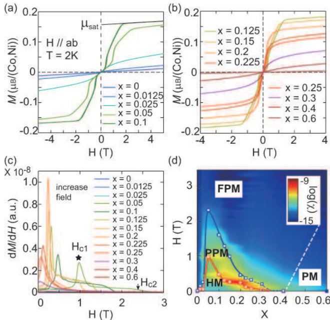
FIG. 3: (a),(b) M(H) for crystals with 0 \leq x \leq 0.6 . (c) dM/dH vs. H for 0 \leq x \leq 0.6 . (d) Magnetic phase diagram with H and x . H_{c1} and H_{c2} are defined in frame (c). H_{c2} is represented as blue dashed curve where it is poorly determined by the data. The white dashed line is a speculative separation (or crossover) between paramagnetic (PM) and field-induced FM states. PPM refers to the partially polarized magnetic state, and FPM means fully polarized magnetic state.
