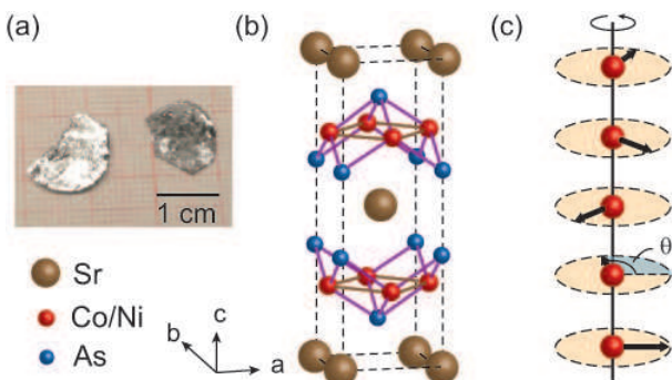
FIG. 1: (a) Single crystals of \text{Sr}(\text{Co}_{1-x}\text{Ni}_x)_2\text{As}_2 . (b) Tetragonal structure of \text{SrCo}_2\text{As}_2 . (c) Helical magnetic structure along the c -axis with a rotation angle \theta between neighboring layers.
