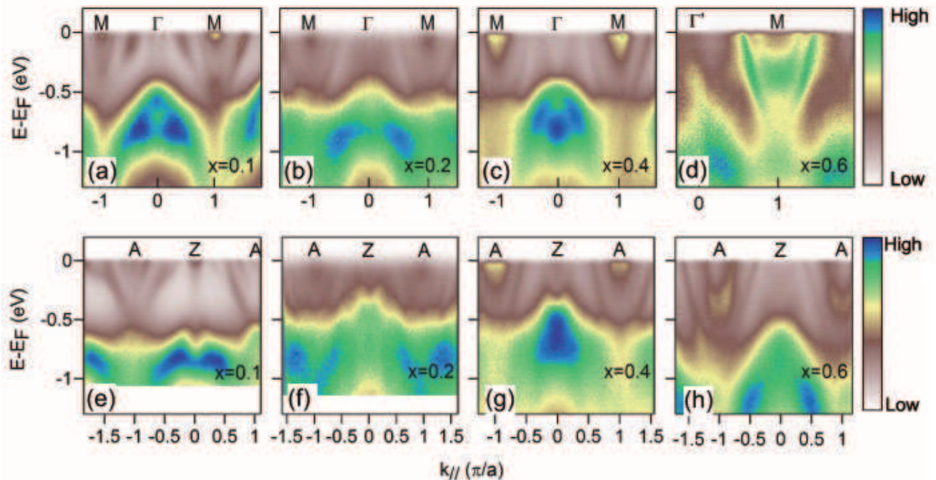
FIG. 10: Intensity plots of the band dispersion along the \Gamma -M (a-d) and Z-A (e-h) directions from ARPES measurements for x = 0.1, 0.2, 0.4, and 0.6 .
