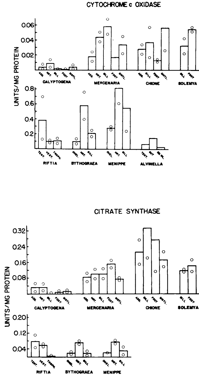
FIGURE 1. Enzymic activities in different tissues of invertebrates from hydrothermal vent and shallow marine habitats. Activities are expressed as international units ( \mu moles substrate converted to product per minute) per mg protein in the supernatant fractions used as sources of enzyme. The heights of the bars indicate the average values for each tissue; the open circles indicate the measured values. In most cases two individuals of a species were measured. The tissues are abbreviated on the abscissa of each graph as follows: add. (adductor muscle), hrt. (heart), mntl. (mantle), tent. (tentacle), vest. (vestimental muscle), troph. (trophosome), chel. (cheliped), bd. wl. (body wall). The habitats of the species are given in Materials and Methods.
