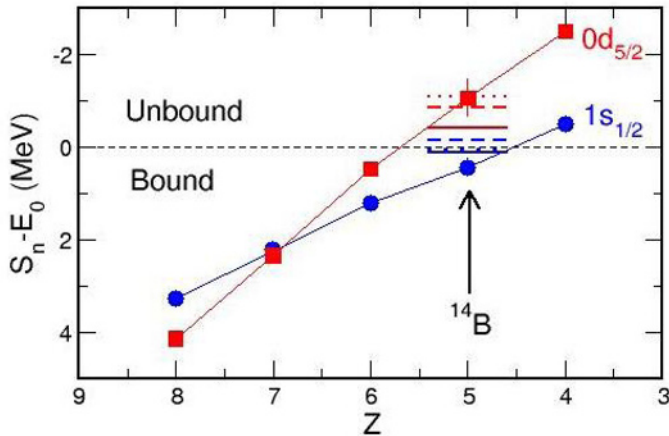
Figure 4. Effective single-particle energies for N=9 isotones as a function of Z .
