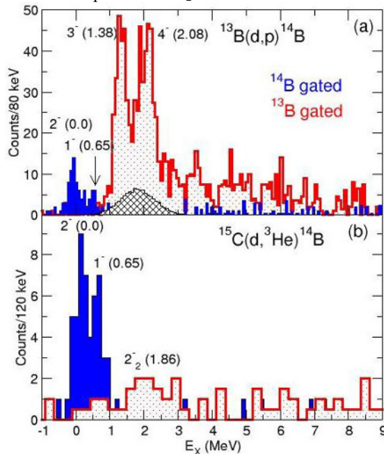
Figure 1. Excitation-energy spectra for the ^{13}\text{B}(d,p)^{14}\text{B} (a) and ^{15}\text{C}(d,^3\text{He})^{14}\text{B} (b) reactions.
