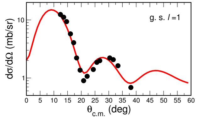
FIG. 9. (Color online) Angular-distribution data for the ^{14}\text{C}(d,^3\text{He})^{13}\text{B}(3/2^-) ground-state transition from Ref. [6]. The curve represents a DWBA calculation described in the text.
