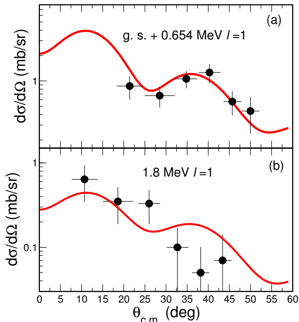
FIG. 12. (Color online) Angular distribution for the (a) 2_1^-1_1^- doublet and (b) 1.8 MeV state in ^{14}\text{B} . The horizontal error bars show the angular range for each point. The DWBA curves represent \ell = 1 transitions as described in the text.
