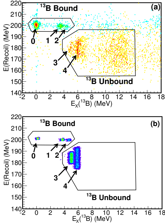
FIG. 8. (Color online) Correlation between boron recoil energy and reconstructed ^{13}\text{B} excitation energy. (a) Data (b) Monte Carlo simulation. The polygons illustrate the regions corresponding to bound and unbound states in ^{13}\text{B} and are not used as event-selection criteria in the analysis. The labels (0)-(4) correspond to excitations in ^{13}\text{B} listed in Table I.
