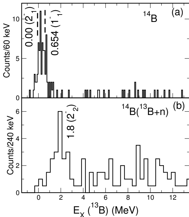
FIG. 7. ^{14}\text{B} excitation-energy spectra from the ^{15}\text{C}(d,^3\text{He})^{14}\text{B} reaction. (a),(b) Particle-bound (unbound) states obtained in coincidence with identified ^{14}\text{B} ( ^{13}\text{B} ) ions.
