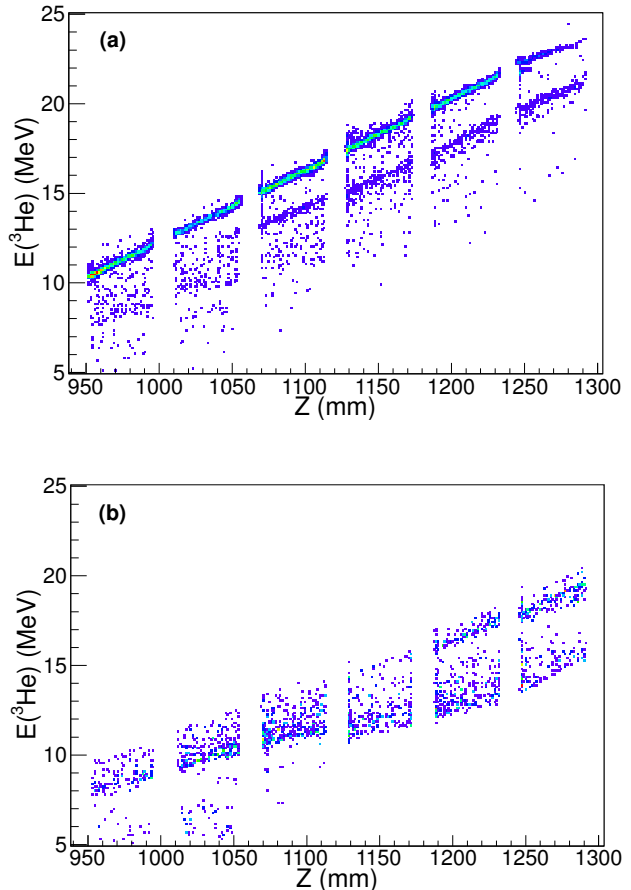
FIG. 3. (Color online) Energy-versus-position spectra for ^3\text{He} particles from the ^{14}\text{C}(d,^3\text{He})^{13}\text{B} reaction. (a) Data for ^3\text{He}+^{13}\text{B} coincidence events. (b) Data for ^3\text{He}+^{12}\text{B} coincidence events. Further analysis on the unbound states includes only data taken for z > 1180 mm.
