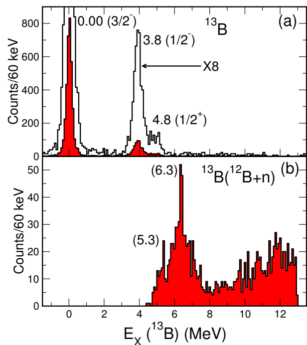
FIG. 6. (Color online) {}^{13}\text{B} excitation-energy spectra from the {}^{14}\text{C}(d,{}^3\text{He}){}^{13}\text{B} reaction. (a) Events in coincidence with identified {}^{13}\text{B} ions with the open histogram displaying the same data multiplied by a factor of 8 to enhance weak transitions. (b) Events in coincidence with identified {}^{12}\text{B} ions.
