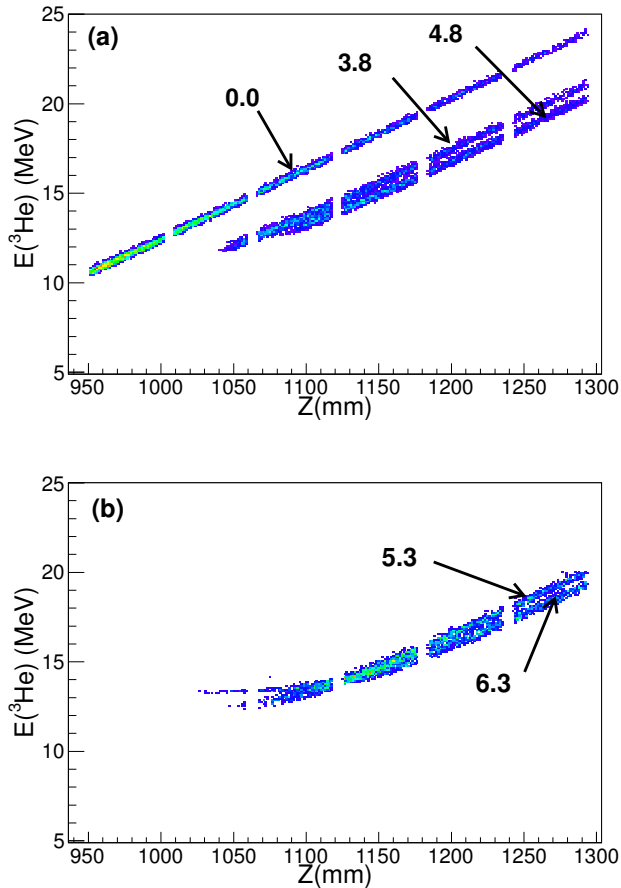
FIG. 4. (Color online) Monte-Carlo simulations of energy-versus-position spectra for {}^3\text{He} particles from the {}^{14}\text{C}(d,{}^3\text{He}){}^{13}\text{B} reaction. (a) Simulated data for {}^3\text{He}+{}^{13}\text{B} coincidence events. (b) Simulated data for {}^3\text{He}+{}^{12}\text{B} coincidence events. The excitation energies used in the calculations are indicated on the figure.
