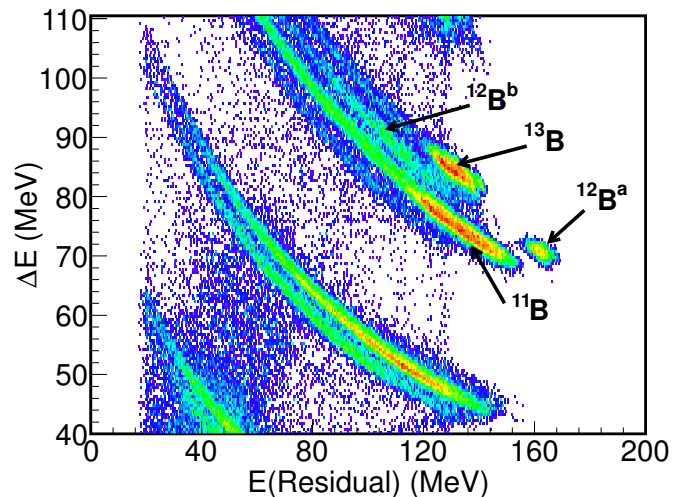
FIG. 2. (Color online) Silicon-detector telescope particle-identification spectrum obtained with the ^{14}\text{C} beam incident on the (\text{CD}_2)_n target. The heavy particles are in coincidence with a particle in the HELIOS PSD array. The groups labeled ^{13}\text{B} and ^{12}\text{B}^b are from particle-bound and unbound states in ^{13}\text{B} ; the groups labeled ^{12}\text{B}^a and ^{11}\text{B} are from particle-bound and unbound states in ^{12}\text{B} from the (d, \alpha) reaction.
