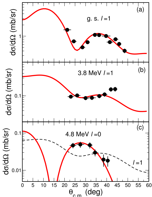
FIG. 10. (Color online) Angular distributions for the (a) 0.0, (b) 3.8 and (c) 4.8 MeV transitions in ^{14}\text{C}(d,^3\text{He})^{13}\text{B} . The curves represent DWBA calculations discussed in the text. For (a), (b) the transitions are \ell = 1 ; for (c) the solid curve corresponds to \ell = 0 . The dashed curve in (c) represents an \ell = 1 transition for comparison. When not visible, the vertical error bars are smaller than the plotting symbols. The horizontal error bars show the angular range for each point.
