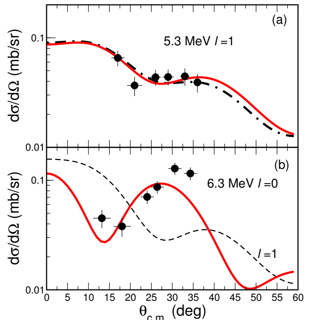
FIG. 11. (Color online) Angular distributions for the (a) 5.3, (b) 6.3 MeV transitions in ^{14}\text{C}(d,^3\text{He})^{13}\text{B} . The curves represent DWBA calculations discussed in the text. The horizontal error bars show the angular range for each point. In (a) the solid and dot-dashed curves correspond to \ell = 1 with J^\pi = 1/2^- or 3/2^- . In (b), the solid and dashed curves represent \ell = 0 and 1 transitions, respectively. The DWBA curves in (b) are for illustration only.
