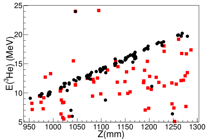
FIG. 5. (Color online) Energy-versus-position spectra for {}^3\text{He} particles from the {}^{15}\text{C}(d,{}^3\text{He}){}^{14}\text{B} reaction. The black circles and red squares correspond to {}^3\text{He}+{}^{14}\text{B} and {}^3\text{He}+{}^{13}\text{B} coincidence events, respectively.
