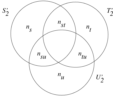
Fig. 1. The cardinalities n_s, n_t, n_u, n_{st}, n_{su} , and n_{tu} .
