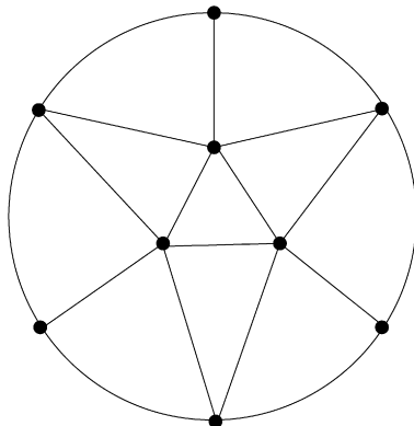
Fig. 3. Simplification and cosimplification are needed.
