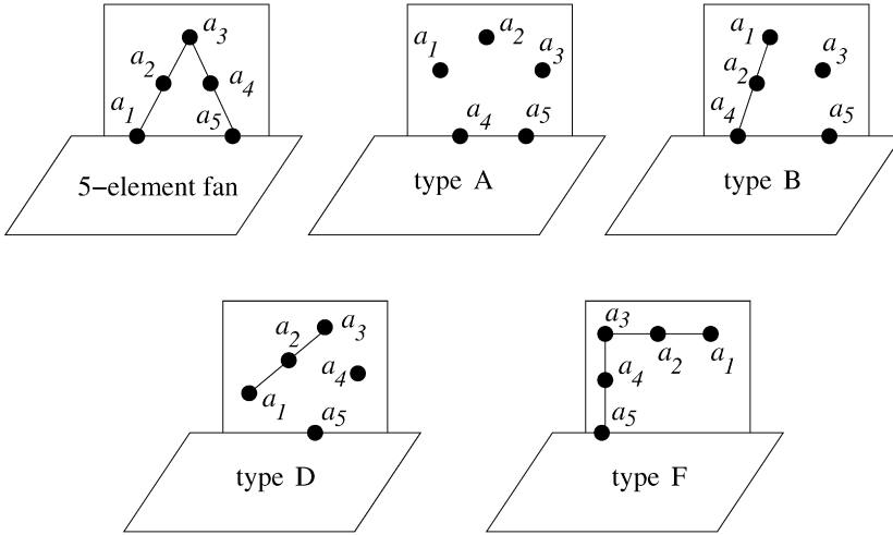
Fig. 2. The five possibilities for the 3-separating set A .
