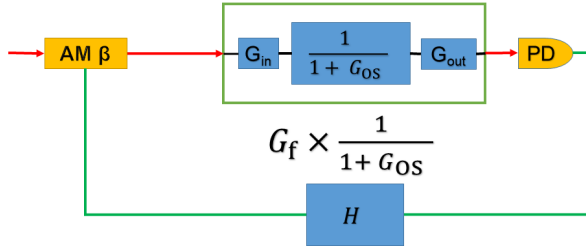
FIG. 3. Loop diagram for the feedback G_f . H is the response of the high pass filter and servo controller, and \beta is the response of the amplitude modulator. \frac{1}{1+G_{\text{os}}} is the closed loop response of the cavity's optical spring system, as shown in Fig 2. G_{\text{in}} = \frac{4T_1}{T^2} \frac{1}{1+\delta^2} is the transfer function of the power input to power inside the cavity with the effect of the detuning taken into account, and similarly G_{\text{out}} = T_2 is the transfer function from cavity power to transmitted power that is measured on the PD. Here T_1 is the transmission of the input mirror, T_2 is the transmission of the microresonator, and T is the total loss of power from the cavity, in the form of transmission, scattering, absorption, etc. G_f = G_{\text{out}} \times \text{PD} \times H \times \beta \times G_{\text{in}} is calculated by using the measurements of the individual transfer functions.
