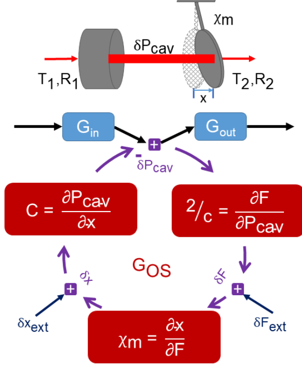
FIG. 2. Detailed loop diagram for the cavity's transfer function. The amplitude modulator adds to the intra-cavity power P_{\text{cav}} . The cavity power converts into radiation pressure force F , which then converts into cantilever displacement x via its mechanical susceptibility \chi_m . The displacement causes a length change for the cavity, leading again to a change in the intracavity power via the cavity response C . This forms a closed loop system.
