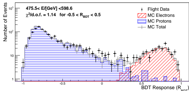
FIG. 3. An example of BDT response distributions in the 476 < E < 599 GeV bin. The reduced chi-square in the BDT response range from -0.5 to 0.5 is obtained as 1.14.
