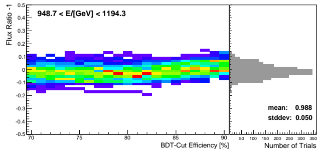
FIG. 4. Stability of BDT analysis with respect to independent training samples and BDT-cut efficiency in the 949 < E < 1194 GeV bin. Color maps show the flux ratio dependence on efficiency, where the bin value (number of trials) increases as color changes from violet, blue, green, yellow to red. A projection onto the Y-axis is shown as a rotated histogram (in gray color).
