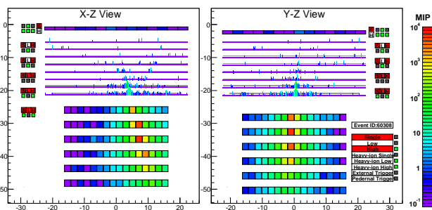
FIG. 2. An example of a 1 TeV electron shower candidate in flight data.
