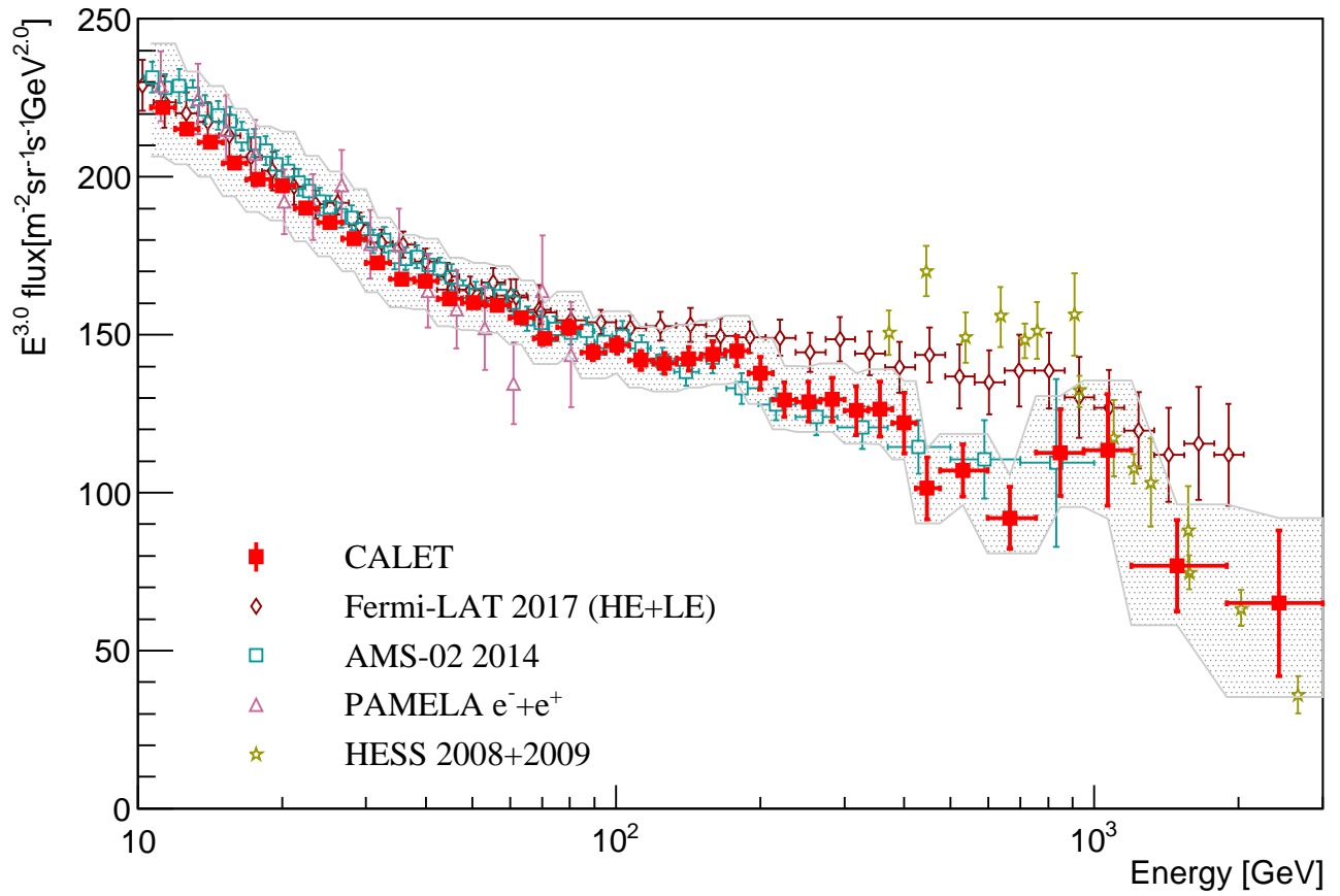
FIG. 6. Cosmic-ray all-electron spectrum measured by CALET from 10 GeV to 3 TeV, where systematic errors (not including the uncertainty on the energy scale) are drawn as a gray band. The measured all-electron flux including statistical and systematic errors is tabulated in Ref. [6]. Also plotted are measurements in space [35–37] and from ground based experiments [38, 39].
