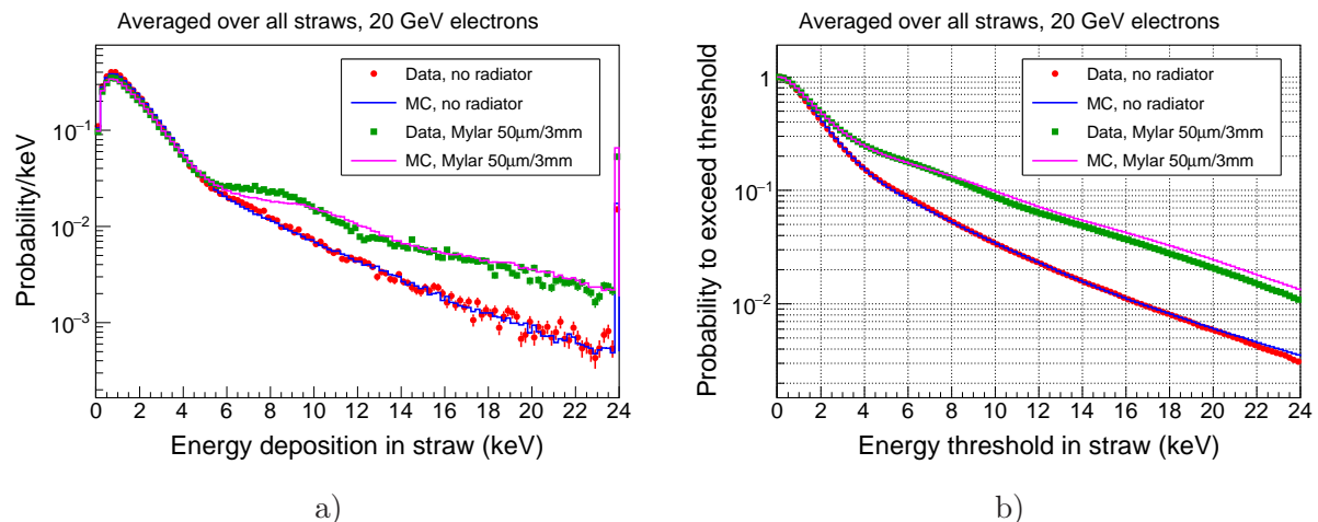
Figure 2. Comparison of experimental and simulated spectra of energy registered in the straws with Mylar radiators and 20 GeV electron beam. a) differential spectra, b) integral spectra (probability to exceed energy threshold). The rightmost bins in the differential spectra include the overflows.
