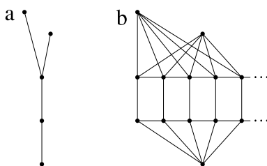
Fig. 1. (a) Tree T . (b) The expansion of T .
