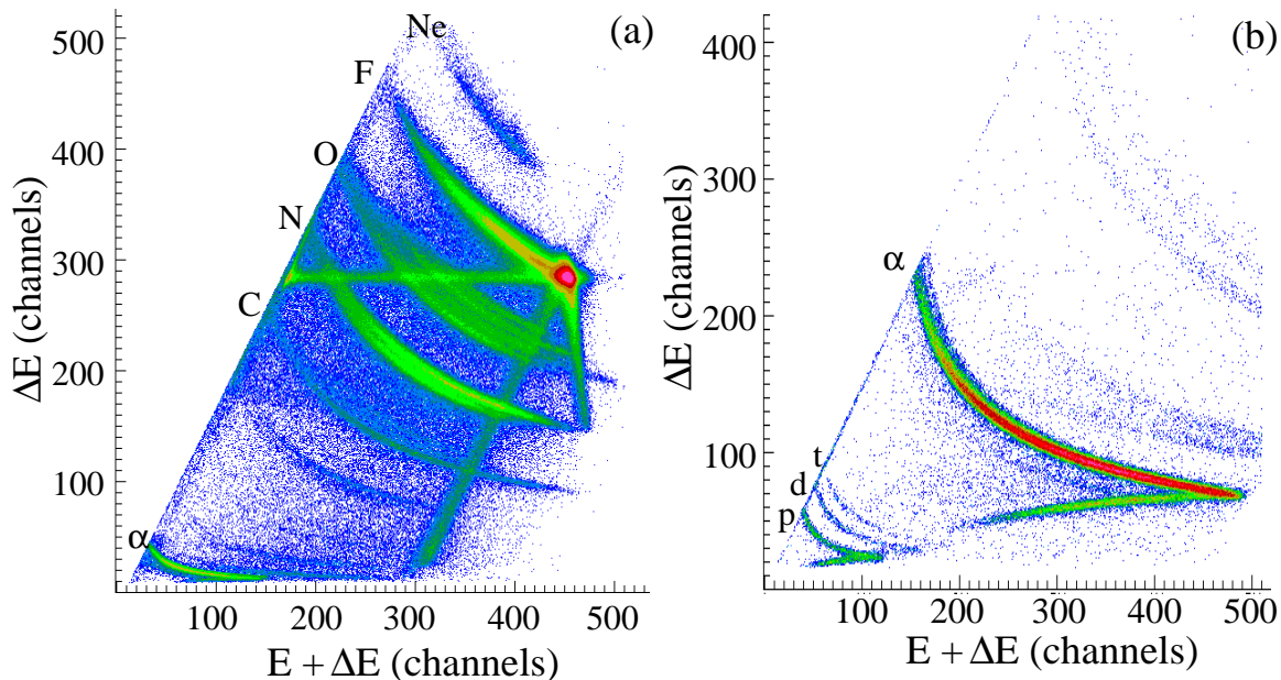
FIG. 2: (Color online) The E_{\text{tot}}-\Delta E spectrum from the experiment for the inner detector (a) and outer detector (b). The loci of nuclei detected by the detectors are indicated. There was complete isotopic separation for H and He and complete Z separation but partial isotopic separation for heavier nuclei.
