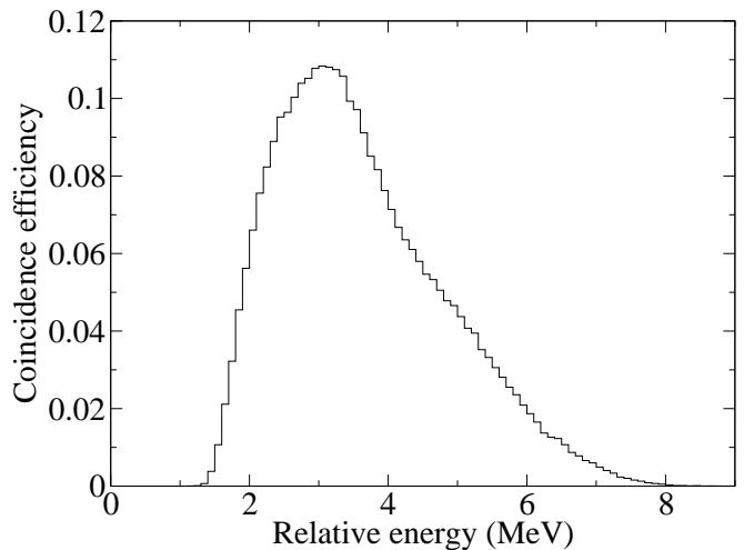
FIG. 6: The calculated coincidence efficiency for our geometry
