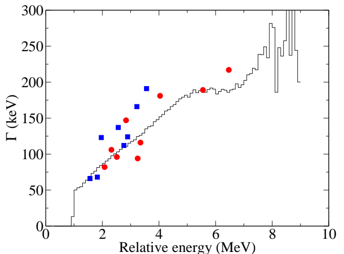
FIG. 7: (Color online) The calculated FWHM resolution for the reconstructed relative energy (solid curve) using our Monte Carlo simulations assuming \alpha + ^{15}\text{O} . Some observed experimental resolutions are indicated for \alpha + ^{15}\text{O} (squares) and \alpha + ^{15}\text{N} (circles).
